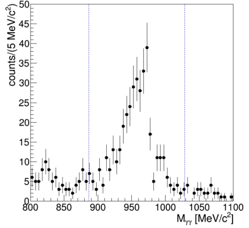
Fig. 1. The 2\gamma invariant mass distribution around the \eta' mass. The region in \pm 4\sigma from the peak is indicated with the blue-dashed lines.
