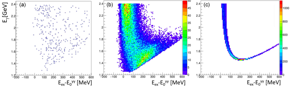
Fig. 4. The two-dimensional event distributions of E_\gamma and E_{\text{ex}} - E_0^{\gamma\gamma} . Here, (a) presents the experimental data, (b) MC simulation data with Fermi motion, and (c) MC data with a proton target.
