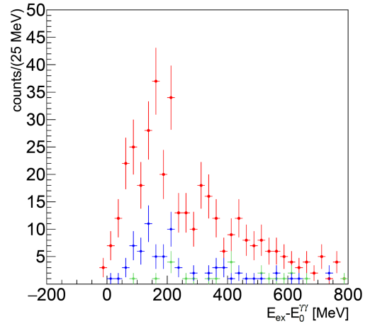
Fig. 2. The missing mass distribution of the \gamma + ^{12}\text{C} \rightarrow p + \eta' + X reaction. The horizontal axis is the excitation energy, E_{\text{ex}} - E_0^{\gamma\gamma} = MM(^{12}\text{C}(\gamma, p_f)) - M_{11\text{B}} - M_{\gamma\gamma} . The red, blue and green histograms indicate events in -4\sigma < M_{\gamma\gamma} < +4\sigma , -8\sigma < M_{\gamma\gamma} < -4\sigma , and +4\sigma < M_{\gamma\gamma} < +8\sigma , respectively.
