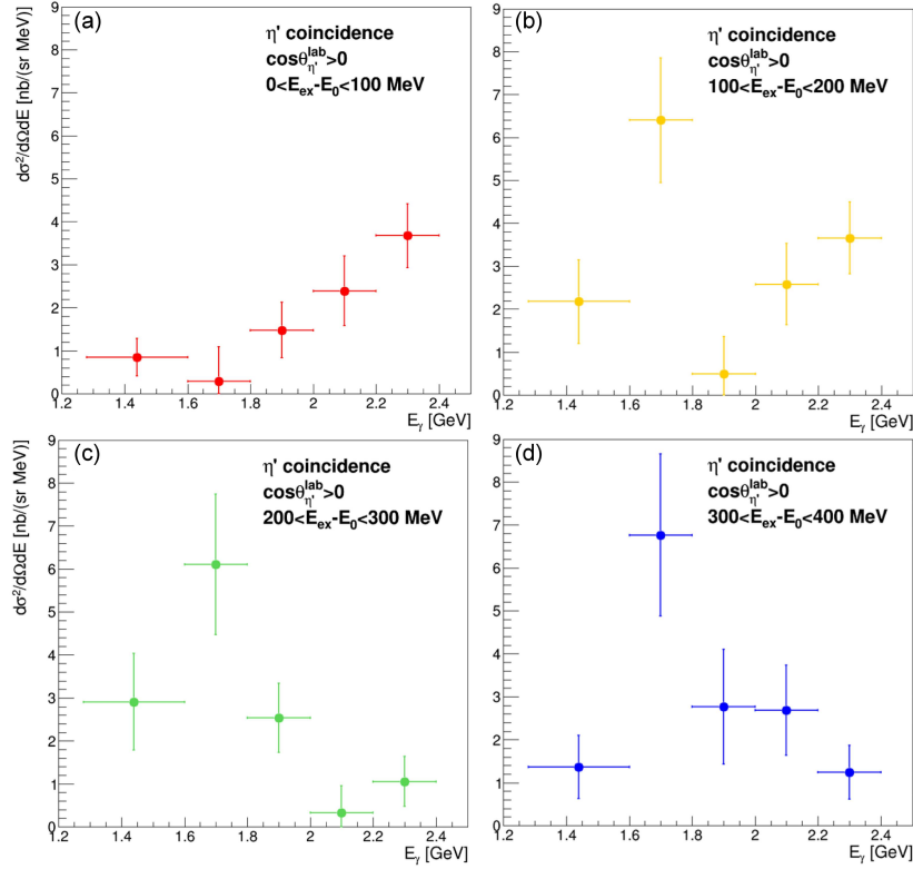
Fig. 3. The E_\gamma dependence of the cross-section of the ^{12}\text{C}(\gamma, p) reaction with simultaneous measurement of an \eta' meson in different E_{\text{ex}} - E_0^{\gamma\gamma} region.
