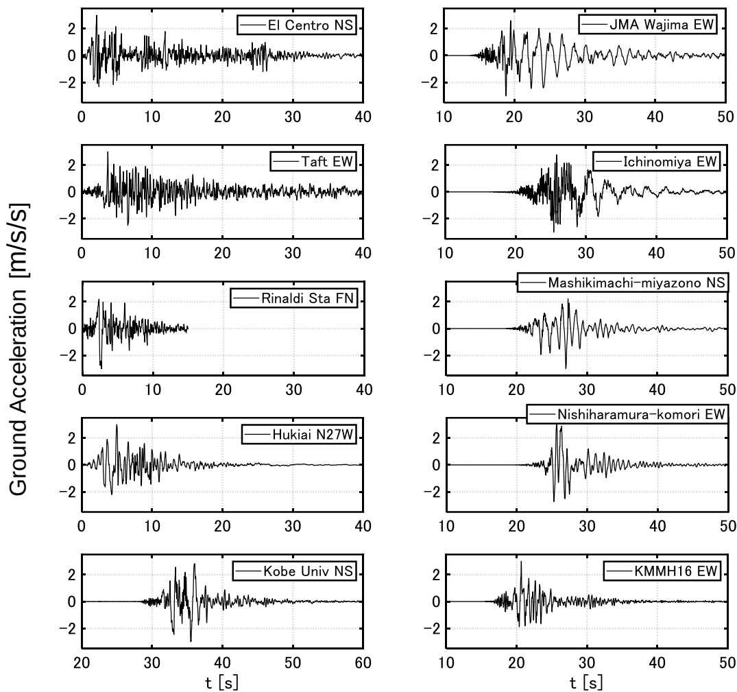
Figure 6 Earthquake ground motions adopted for IDA
