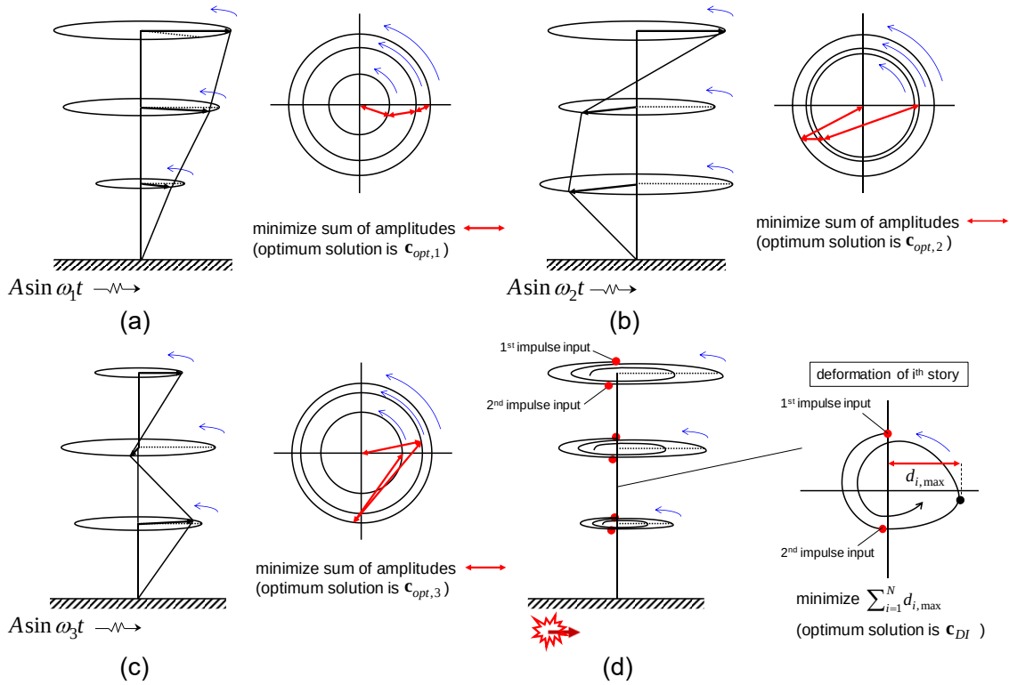
Figure 1 Schematic diagram of criteria of optimal damper designs, (a) Transfer function amplitude at lowest natural frequency, (b) Transfer function amplitude at second natural frequency, (c) Transfer function amplitude at third natural frequency, (d) Sum of maximum interstory drifts under critical double impulse
