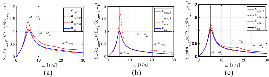
Figure 5 Sum of transfer functions of interstory velocity \sum_{l=1}^N \omega |\delta_l(\mathbf{c}_{add}, \omega)| / \sum_{l=1}^N \omega_1 |\delta_l(\mathbf{c}_{opt,1}, \omega_1)| normalized for 1-st mode optimal design model, (a) Model 1, (b) Model 2, (c) Model 3
