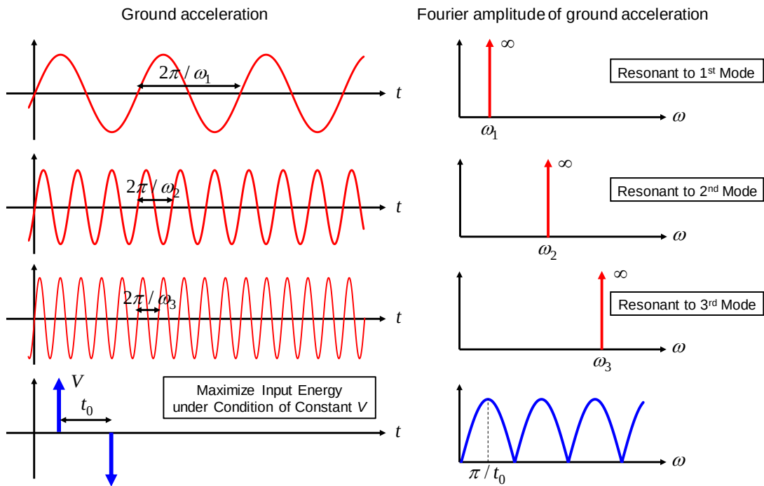
Figure 2 Inputs used for respective optimal damper designs
