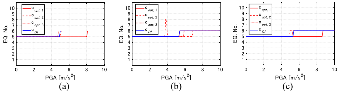
Figure 9 Critical earthquake ground motion numbers for IDA, (a) Model 1, (b) Model 2, (c) Model 3
