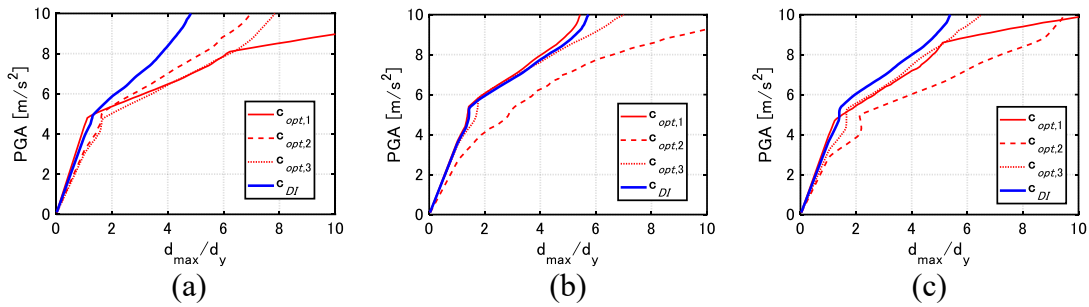
Figure 8 Application of IDA: Maximum interstory drift with respect to peak ground acceleration, (a) Model 1, (b) Model 2, (c) Model 3
