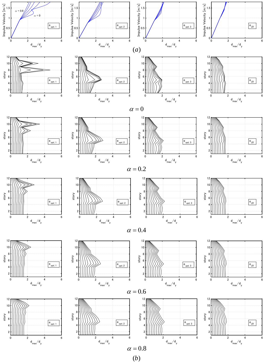
Figure 12 DIP analysis for Model 3: Maximum interstory drift, (a) Maximum interstory drift with respect to input velocity level, (b) Maximum interstory drift for various input velocity levels v = 0.2-1.8\text{m/s} and various second stiffness ratio after yielding
