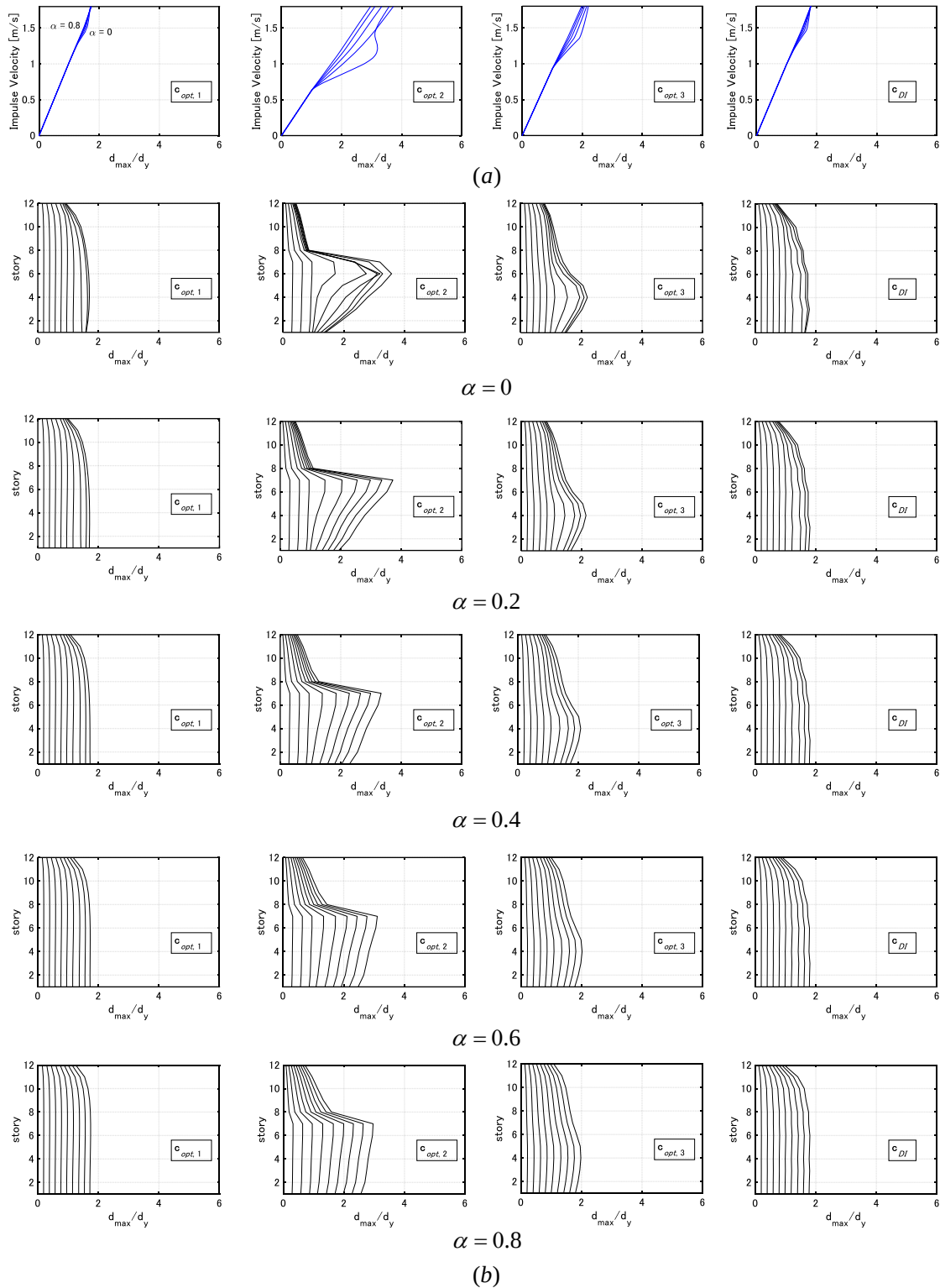
Figure 11 DIP analysis for Model 2: Maximum interstory drift, (a) Maximum interstory drift with respect to input velocity level, (b) Maximum interstory drift for various input velocity levels V = 0.2-1.8\text{m/s} and various second stiffness ratio after yielding
