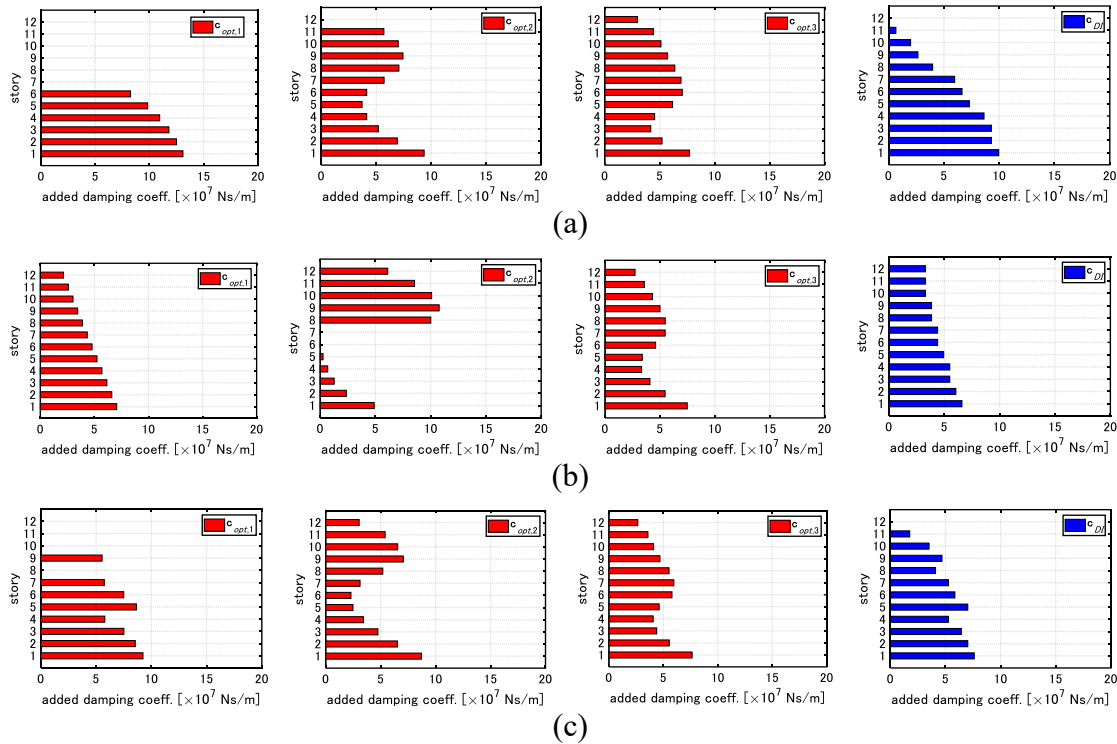
Figure 4 Optimal damper distribution c_{opt,1} , c_{opt,2} , c_{opt,3} , c_{DI} , (a) Model 1 (Uniform story stiffness distribution), (b) Model 2 (Straight-line lowest eigenmode), (c) Model 3 (Uniform story stiffness distribution at every four stories)
