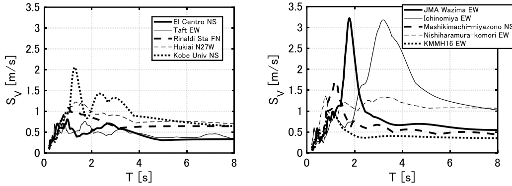
Figure 7 Velocity response spectra for damping ratio h = 0.05 of recorded ground motions normalized by \text{PGA} = 3[\text{m/s}^2] and used for IDA procedure
