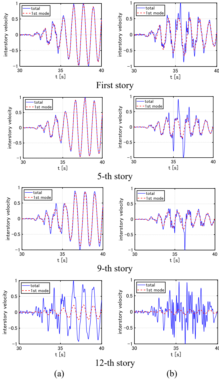
Figure 3 Elastic eigenmode expansion of interstory velocity of elastic structure and elastic-plastic structure under Kobe Univ. NS (1995), (a) Elastic structure, (b) Elastic-plastic structure
