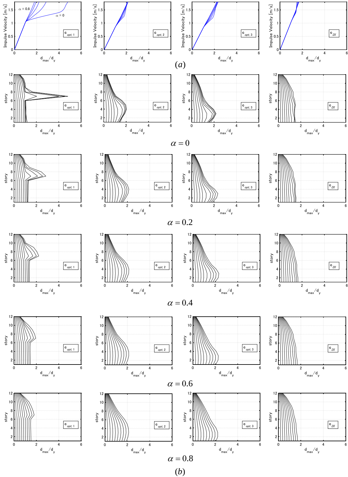
Figure 10 DIP analysis for Model 1: Maximum interstory drift, (a) Maximum interstory drift with respect to input velocity level, (b) Maximum interstory drift for various input velocity levels V = 0.2-1.8\text{m/s} and various second stiffness ratio after yielding
