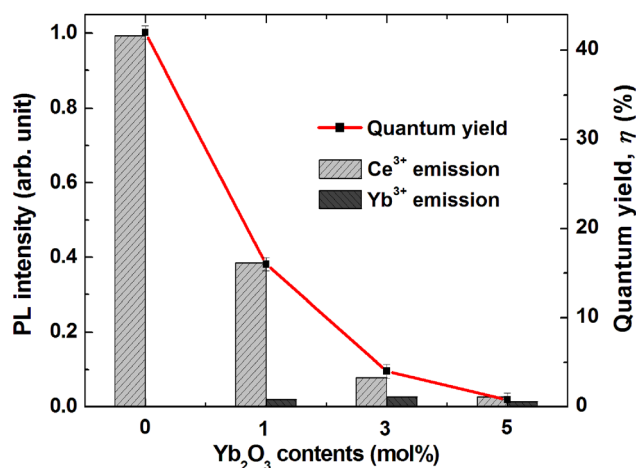
FIG. 4. PL intensity histogram and absolute quantum yield as a function of \text{Yb}_2\text{O}_3 concentration.
