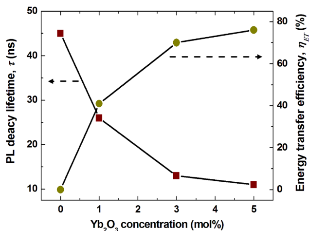
FIG. 6. \text{Ce}^{3+} PL decay lifetime and \text{Ce}^{3+} \rightarrow \text{Yb}^{3+} energy transfer efficiency as a function of \text{Yb}_2\text{O}_3 concentration.
