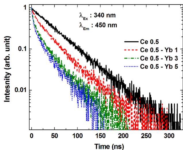
FIG. 5. \text{Ce}^{3+} PL decay curves in \text{Ce}^{3+} singly and \text{Ce}^{3+}\text{-Yb}^{3+} codoped glasses.
