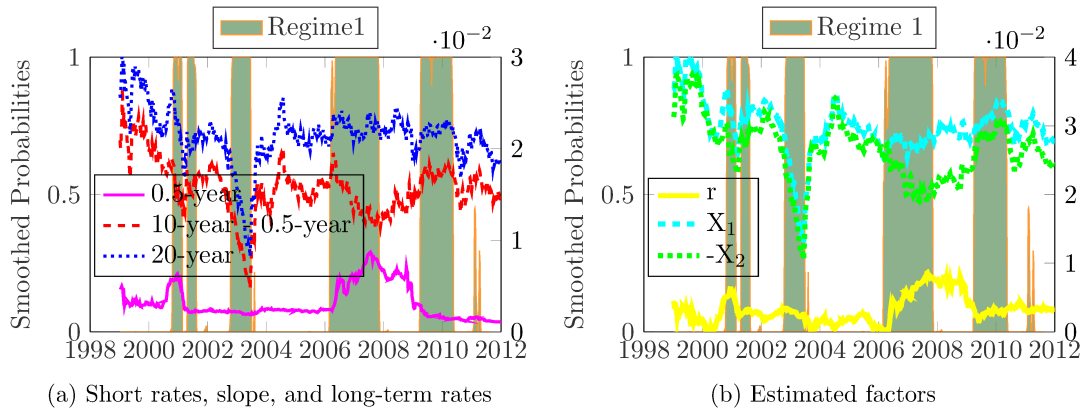
Figure 3: Smoothed probabilities of regime 1 (RSDNS)
