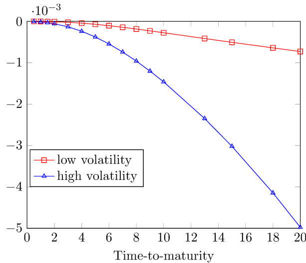
Figure 6: RSAFNS's adjustment term
