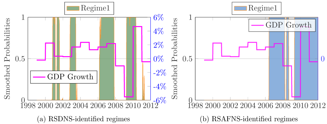
Figure 4: Smoothed probabilities of regime 1 and GDP growth
