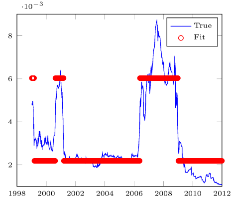
Figure 2: Fitting MS mixed normal distribution model to 6-month yields.
