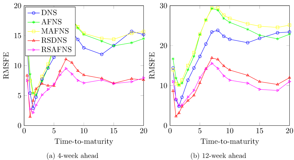
Figure 10: Root mean square forecast errors
