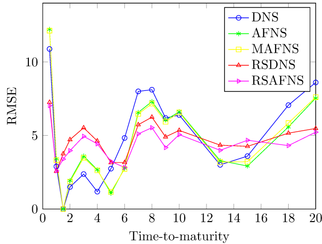
Figure 9: Root mean square errors
