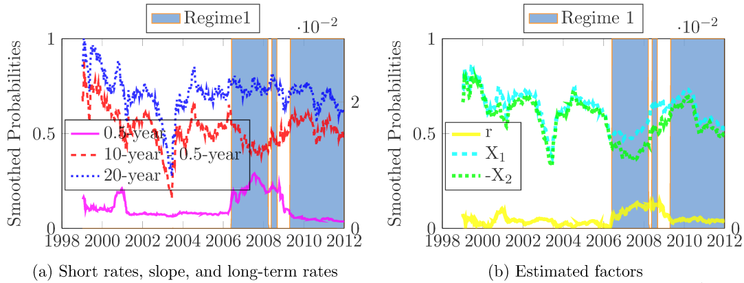
Figure 5: Smoothed probabilities of regime 1 (RSAFNS)
