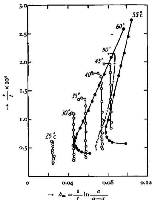
Fig. 4. \frac{x}{t} - \frac{1}{t} \ln \frac{a}{a-x} relation for the reactions at various temperatures.
