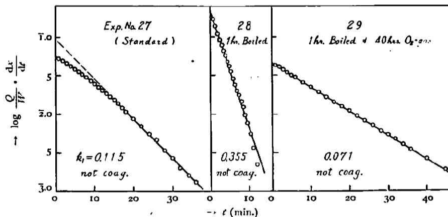
Fig. 7. The reactions with the boiled sol. (c). Initial conc. of \text{H}_2\text{O}_2 : 0.029 g.-mol./litre. Conc. of Pt-sol. (No. 5): 10 \times 10^{-4} g.-atom/litre. Temperature: 25°C.
