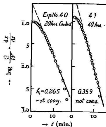
Fig. 12. The reactions with the cooled sol.
