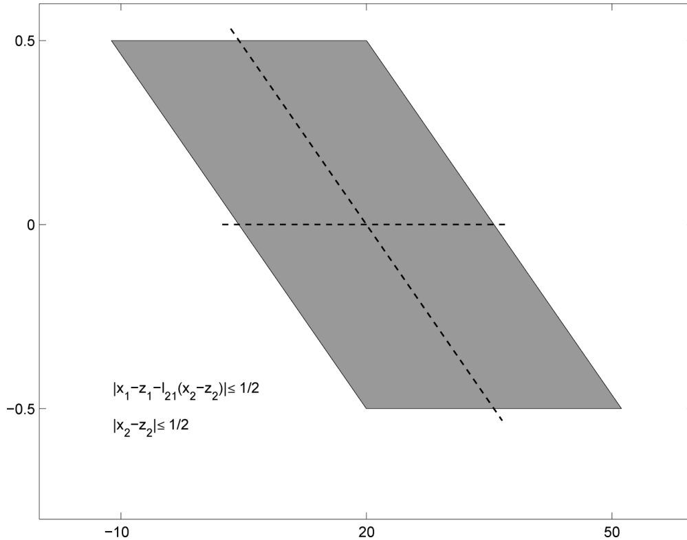
Fig. 4. Illustrated domain of integration used for computing the probability that the integer bootstrapped estimator correctly produces the integer vector \mathbf{z} of the model.
