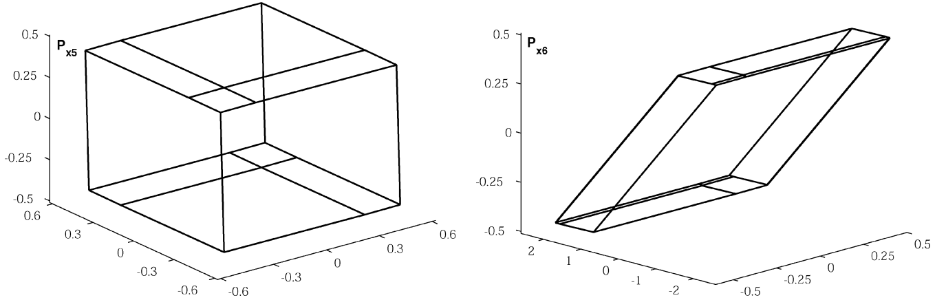
Fig. 2. The orientations, shapes, and actual sizes of the two three-dimensional Voronoi cells.
