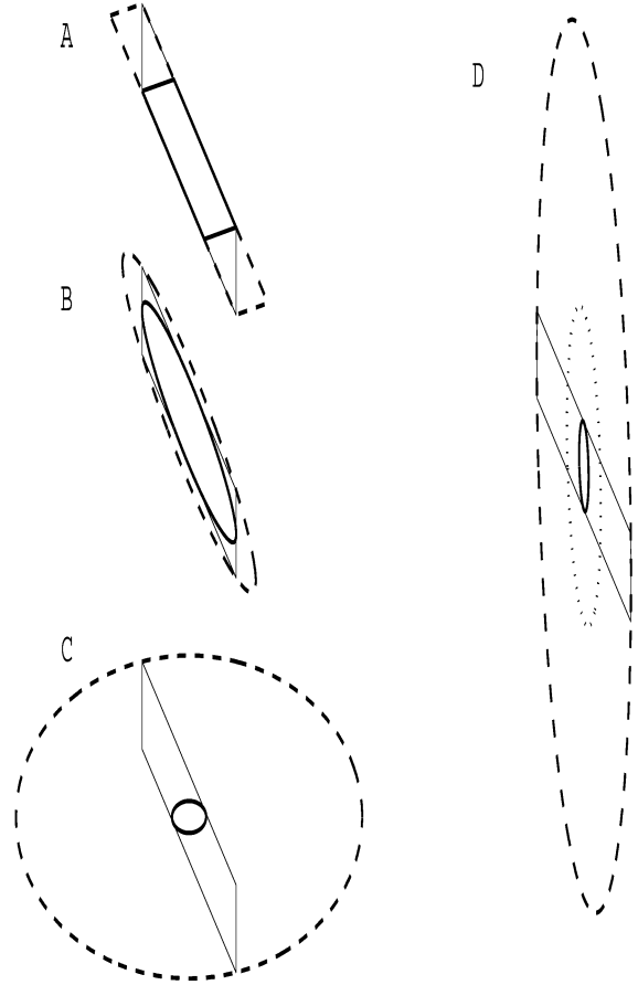
Fig. 3. Fitting the Voronoi cell V_0 by using the different types of figures: A—rectangular type; B—first ellipsoidal type with maximum volume; C—spherical type; and D—second ellipsoidal type with the shapes fixed by the matrix P_{x1} . The Voronoi cell V_0 is shown in these fittings in solid line. Thick dashed and thick solid lines show the upper and lower bounds of the Voronoi cell V_0 for each type of fitting, respectively. Thick dotted line in subplot D shows the ellipse with the same area as that of the Voronoi cell.
