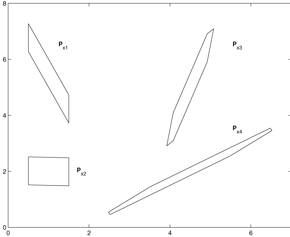
Fig. 1. The orientations, shapes and actual sizes of the four Voronoi cells.
