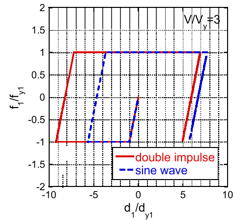
FIGURE A3 | Comparison of first-story restoring-force characteristic under the double impulse and the corresponding sinusoidal wave.
