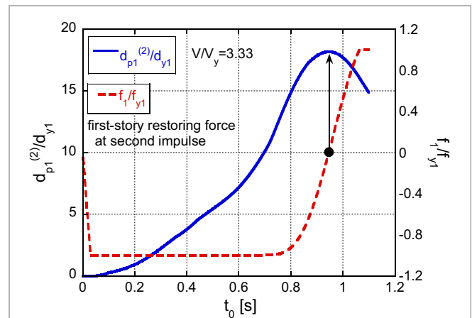
FIGURE 22 | Plot of d_{p1}^{(2)}/d_{y1} and f_1/f_{y1} (restoring force in the first story at the second impulse) with respect to the timing of the second impulse.
