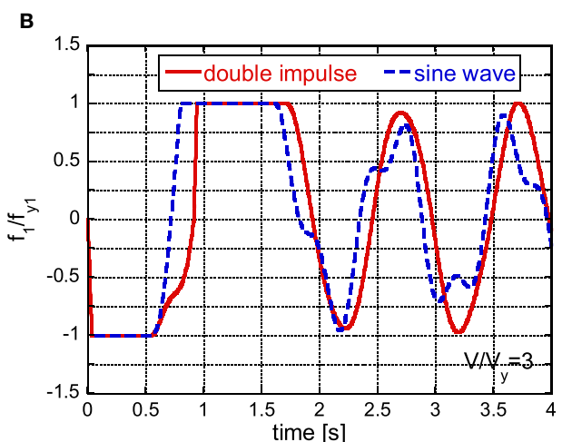
FIGURE A2 | Comparison of time histories of the first-story interstory drift and the first-story restoring force under the double impulse and the corresponding sinusoidal wave. (A) First-story interstory drift. (B) First-story restoring force.
