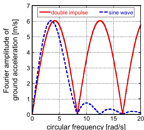
FIGURE A1 | Adjustment of input level of double impulse and the corresponding one-cycle sinusoidal wave based on Fourier amplitude equivalence.
