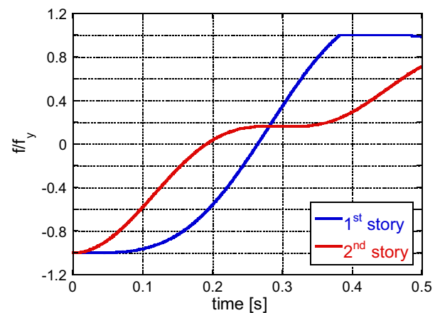
FIGURE 16 | Time histories of the restoring forces in the first and second stories starting from the phase (A).
