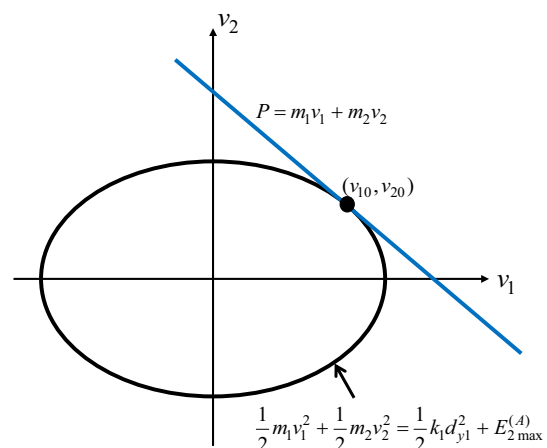
FIGURE 8 | Tangential line of the ellipse (m_1 v_1^2 / 2) + (m_2 v_2^2 / 2) = D at the point (v_{10}, v_{20}) .
