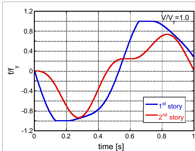
FIGURE 3 | Example of the time histories of the restoring forces in the first and second stories for a model of equal mass, equal story stiffness, and equal yield interstory drift subjected to the single impulse at t = 0 with V/V_y = 1.0 .
