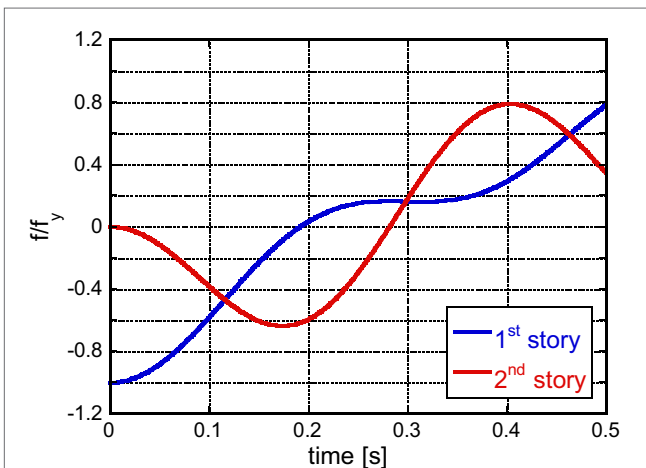
FIGURE 20 | Time histories of the restoring forces in the first and second stories starting from the phase (A).
