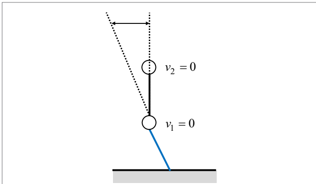
FIGURE 19 | Deformation mode and velocity at the phase (A) (lower bound case).
