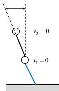
FIGURE 15 | Deformation mode and velocity at the phase (A) (upper bound case).
