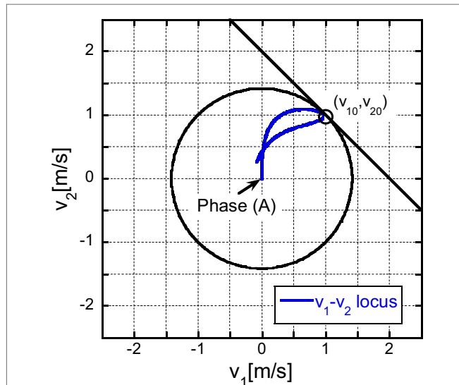
FIGURE 17 | Velocity (first-story mass)-Velocity (second-story mass) plane for variable motion of masses attaining the maximum sum of momenta (tangential line) by the convex model and the actual motion of masses starting from the phase (A) (only the first impulse is given).
