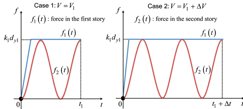
FIGURE A4 | Time histories of the restoring forces in the first and second stories up to the phase (A).
