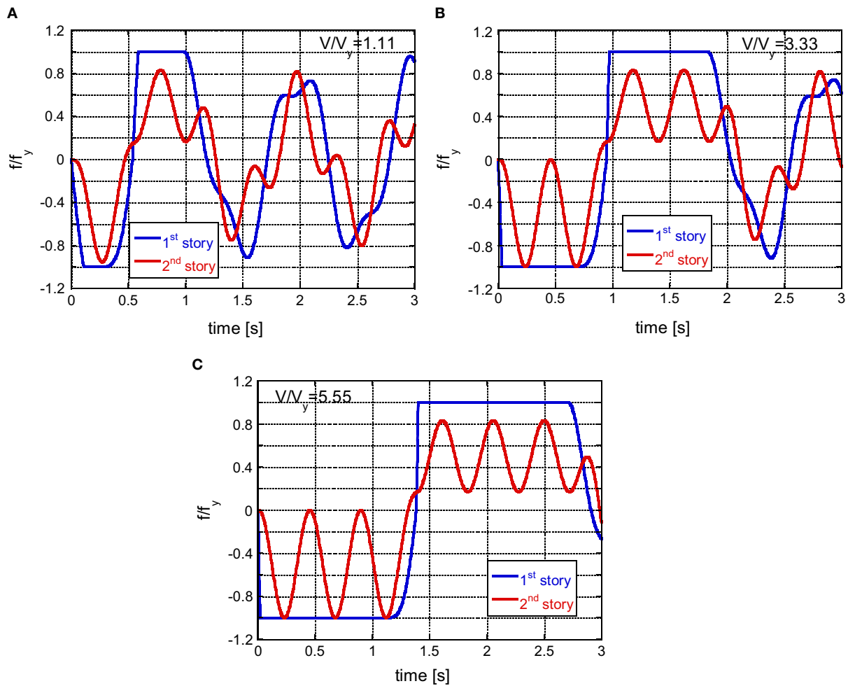
FIGURE 14 | Time histories of the restoring forces in the first and second stories for the same 2DOF model subjected to the double impulse with V/V_y = 1.11, 3.33, 5.55 . (A) V/V_y = 1.11 ( t_{0c} = 0.535 [s]). (B) V/V_y = 3.33 ( t_{0c} = 0.946 [s]). (C) V/V_y = 5.55 ( t_{0c} = 1.384 [s]).
