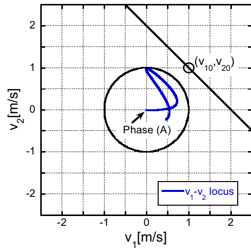
FIGURE 21 | Velocity (first-story mass)–Velocity (second-story mass) plane for variable motion of masses bounded by shrunk circle and the actual motion of masses starting from the phase (A) (only the first impulse is given).
