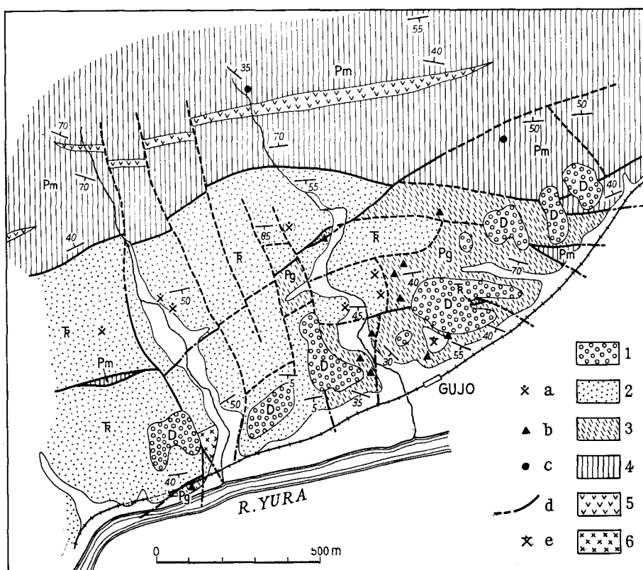
Fig. 2. Geologic map of the vicinity of Gujo in the Maizuru Belt, Southwest Japan (simplified from NAKAZAWA and NOGAMI, 1962).
