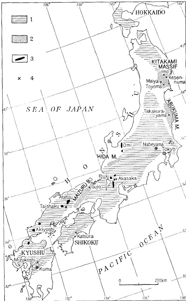
Fig. 1. Schematic lithofacies map of the Permian in Japan, and main fossil localities of bivalves (x).
