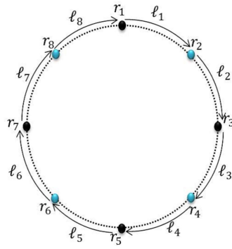
Figure 2: \ell_1 = \ell_2 = \dots = \ell_8 .
