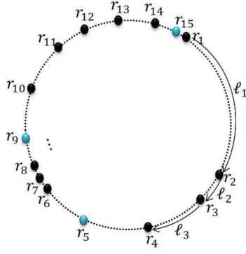
Figure 1: \ell_1 is larger than \ell_i for any i = 2, 3, \dots, 15 .
