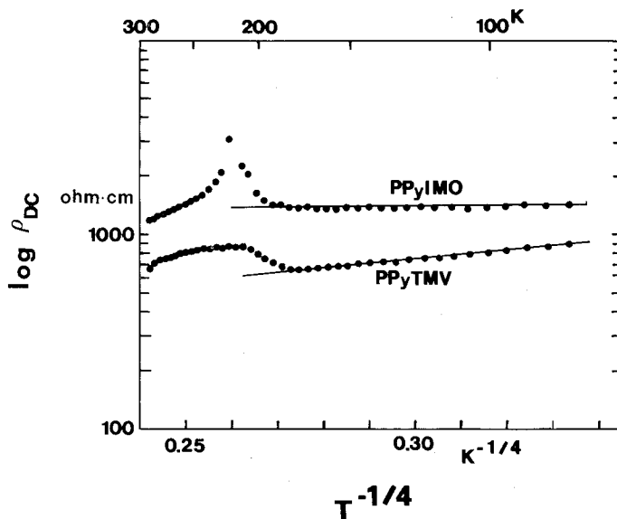
Fig. 9 \log(\rho_{DC}) vs. T^{-1/4} plot for PPyIMO and PPyTMV based on the variable range hopping model.
