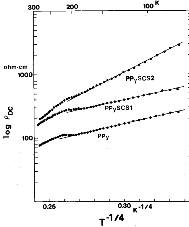
Fig. 6. \log(\rho_{DC}) vs. T^{-1/4} plot based on Mott's variable range hopping in three dimension. Better linearity in a wider temperature region is observed than the cases of Figs. 4 and 5.
