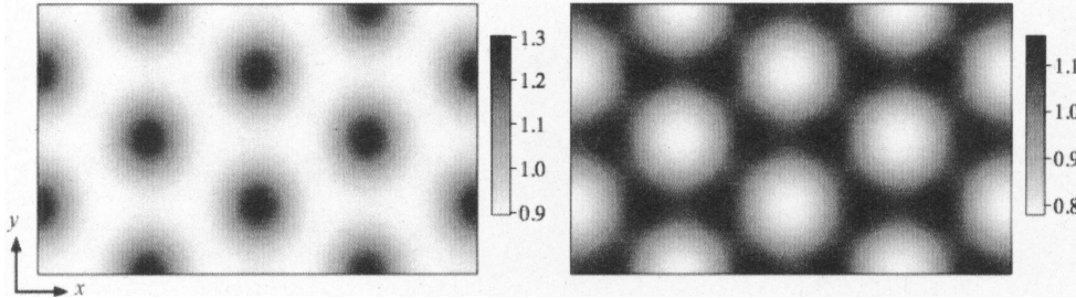
Figure 2: Dot and hexagonal pattern formation of solutions to the system (E). A dot pattern (left) and a hexagonal pattern (right) [9, 16]. In actual phenomena, some dot patterns have been observed; on the other hand, hexagonal patterns have not been observed, as far as the authors know.
