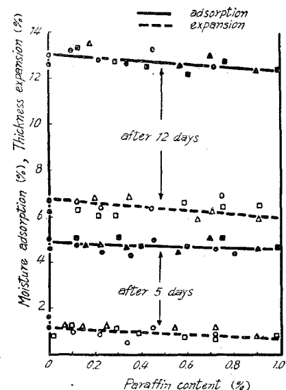
Fig. 6 : Effects of paraffin content on the moisture adsorption and thickness expansion of chipboard in a desiccator saturated by moisture at 7° C.
