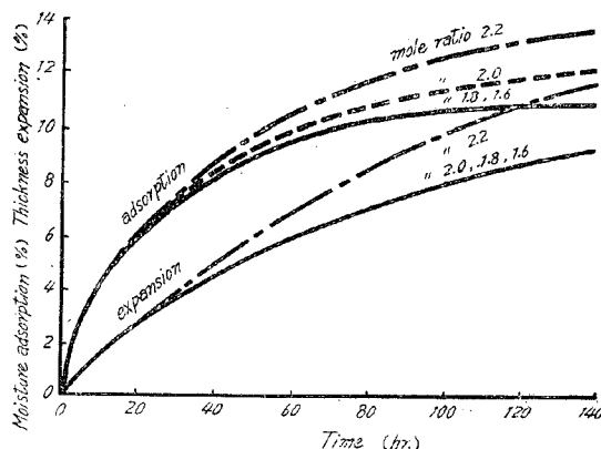
Fig. 15 : Effects of molar ratio of urea resin on the moisture adsorption and thickness expansion of chipboard in a desiccators saturated by moisture at 40° C.
