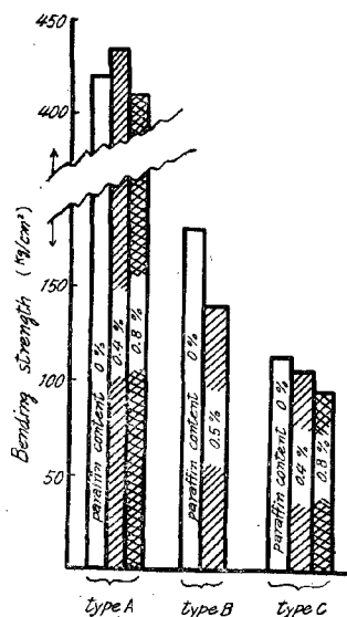
Fig. 9 : Effect of paraffin on the bending strength of chipboard made of various shavings.
