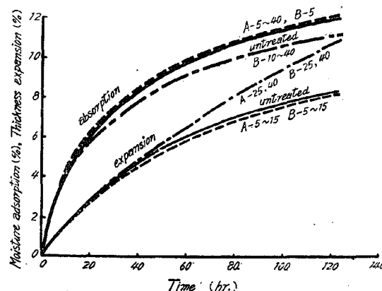
Fig. 11 : Effects of heat treatment of shavings on the moisture adsorption and thickness expansion of chipboard. (40° C.)
