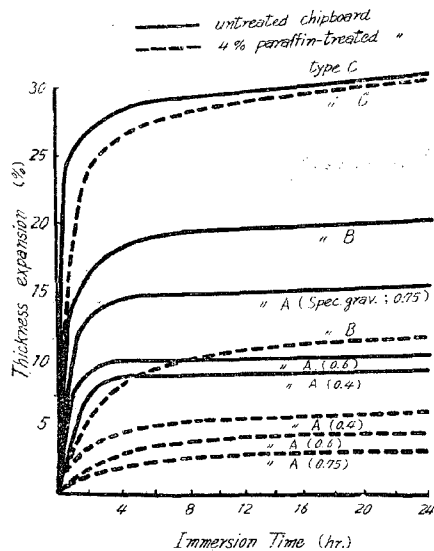
Fig. 4 : Effects of paraffin on thickness expansion of chipboard varied in specific gravity or type of shavings.
