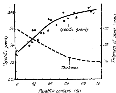
Fig. 8 : Effects of paraffin content on the specific gravity and thickness of chipboard.
