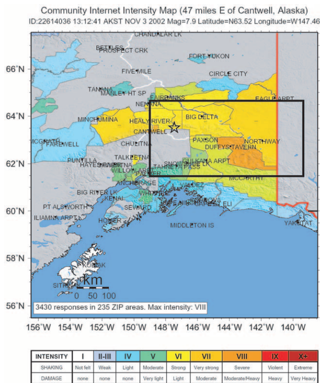
Figure 12. Community Internet Intensity Map by the USGS (Wald et al. , 1999a). This map is available on the Internet at the USGS Web site ( http://pasadena.wr.usgs.gov/shake/ak/STORE/X22614036/ciim_display.html ).
