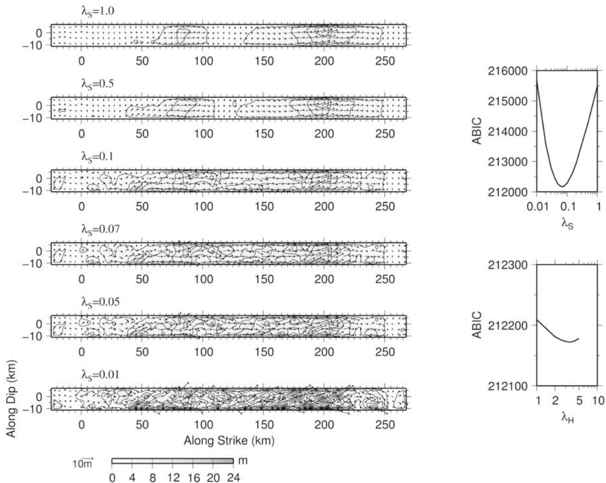
Figure 7. (left) The variation of final slip distribution on the fault plane with different smoothing strengths \lambda_S . The interval between the contours is 2 m. (right) The variation of ABIC due to two hyperparameters \lambda_S and \lambda_H . In the upper figure, \lambda_H is fixed at 3.5. In the bottom figure, \lambda_S is fixed at 0.07.
