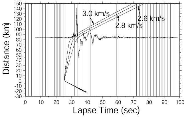
Figure 2. S -phase arrival time curves at PS10 from each subfault with a uniform rupture velocity. The observed east-west velocity waveform at PS10 is also shown. Cases for a rupture velocity of 2.6, 2.8, and 3.0 km/sec are shown. To explain the phase corresponding to the dislocation of the fault, the average rupture propagation velocity between the hypocenter and the nearest part from PS10 was estimated to be 2.8 km/sec.
