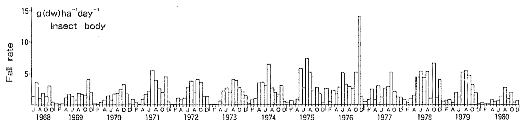
Fig. 7. Seasonal fluctuations in the fall rates of insect bodies in fir-hemlock mixed stand
