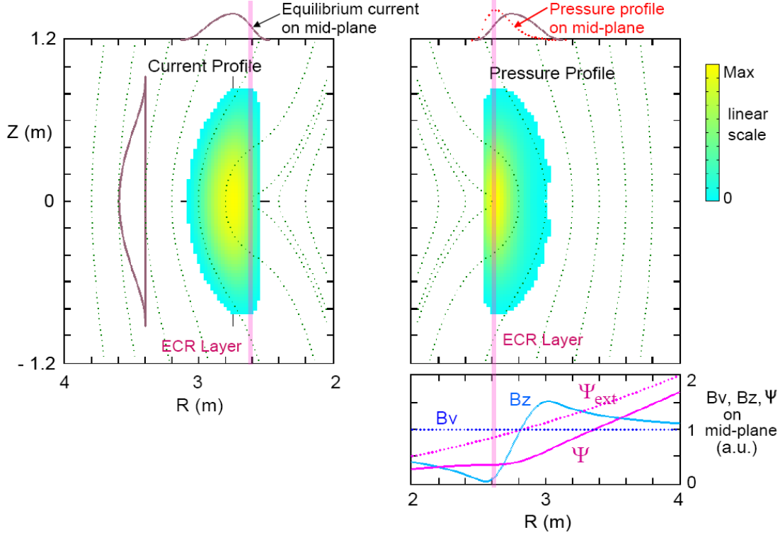
Figure 14. Open field equilibrium modeled for experiments in large tokamaks. R_0=2.8 m, a=0.3 m, b=0.9 m, \alpha=1.8 , \kappa=3 , \delta=0.5 , \sigma=-0.2 , I_{EQL}=-5000 A, B_V=30 G, B_\phi=34200 G at R=3 m, j_{peak}=16.3 kAm ^{-2} , p_{peak}=82.6 Pa ( n_{epeak}=8 \times 10^{18} m ^{-3} , T_{epeak}=65 eV)
