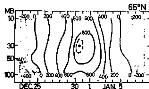
Fig. 17b: The same as Fig. 17a, except vertical-time section at 65^\circ N from 100 mb to 10 mb.
