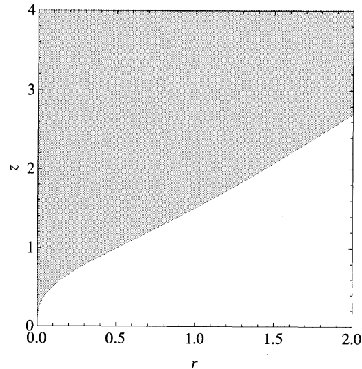
Fig 5: Set defined by \psi(r, z)
