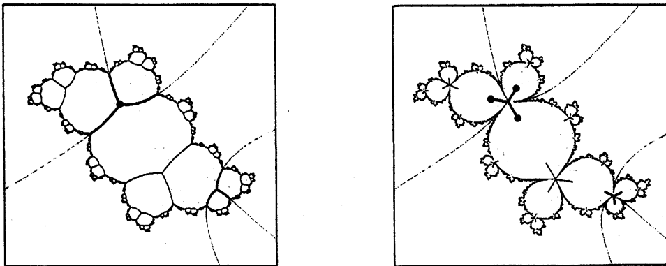
Figure 8: The external rays of angles \{1/7, 2/7, 1/7\} and \{1/28, 23/28, 25/28\} are also drawn in.
