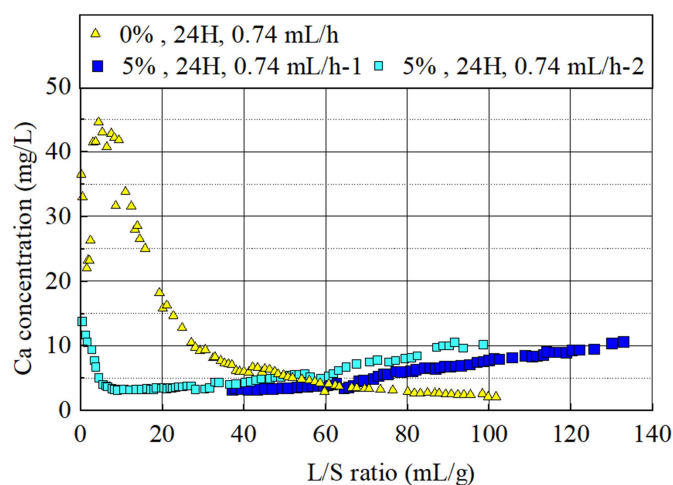
Fig. 5.16 Effluent Ca concentration for 0% and 5% cases under 24-hour contact
