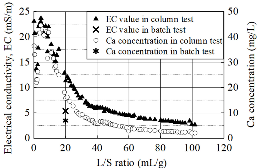
Fig. 4.10 Electrical conductivity for mix proportion of 0% case in column and batch test along with effluent Ca concentration in column test
