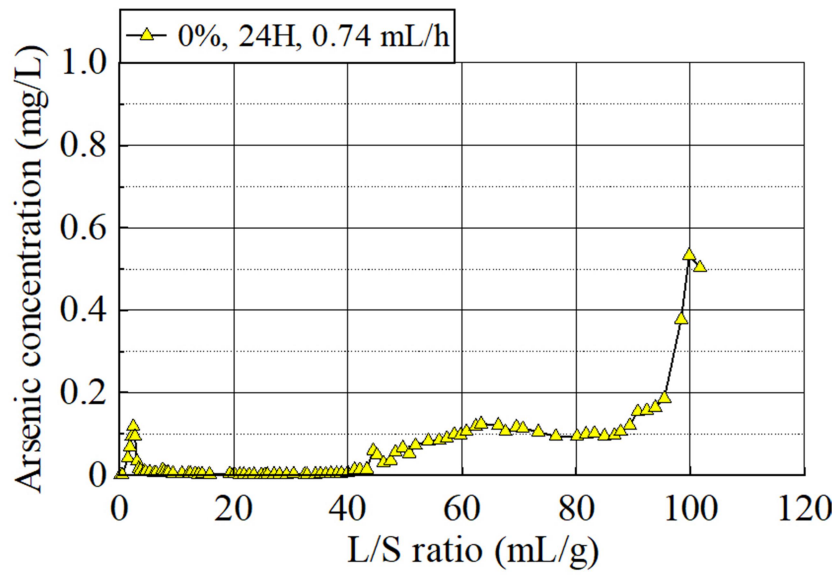
Fig. 4.6 Effluent As concentration for mix proportion of 0%, flow rate of 0.74 mL/h
