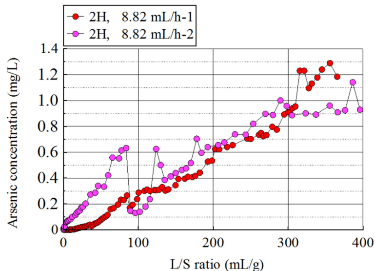
(b) Effluent As concentration of repeated 2-hour contact cases
