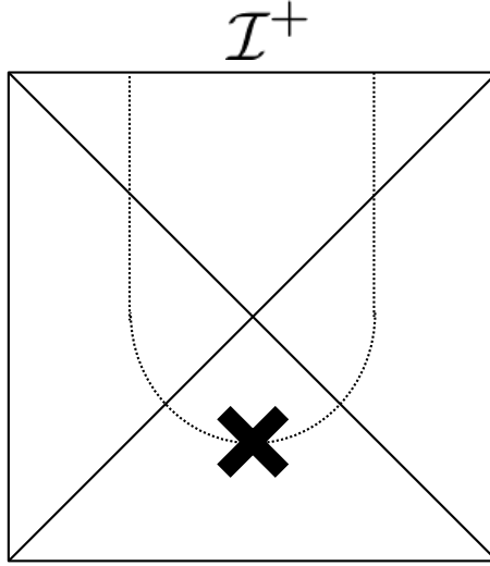
Figure 4.2: Time-like surface in dS spacetime. The mark X means that the surface cannot be closed.
