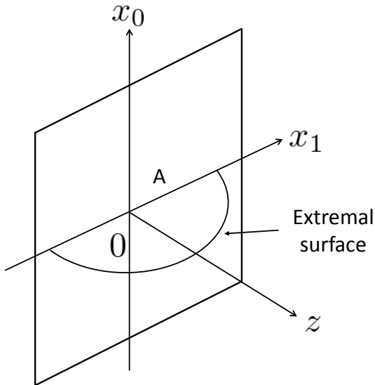
Figure 3.6: Set-ups of a finite interval and extremal surface in \text{AdS}_3 .
