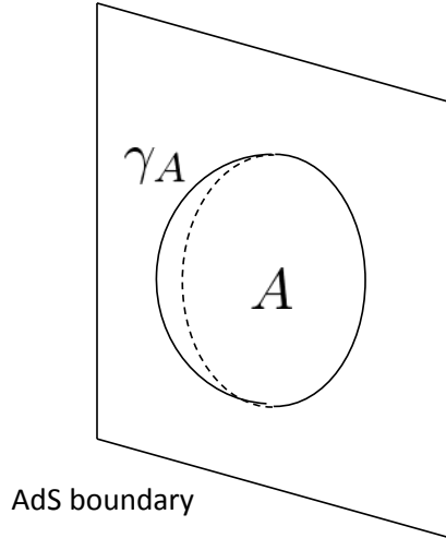
Figure 3.5: Ryu-Takayanagi formula. In this figure, the time-direction is not drawn. The extremal surface \gamma_A dips in the interior of AdS spacetime.
