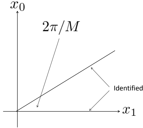
Figure 3.4: \mathbb{R}^2/\mathbb{Z}_M . These two lines are identified.
