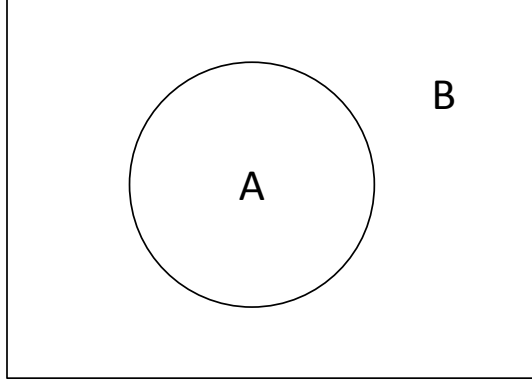
Figure 3.1: Division of the time-slice into the region A and the region B . It is not necessary for the region A to be connected.
