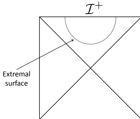
Figure 4.1: Extremal surface in dS spacetime.
