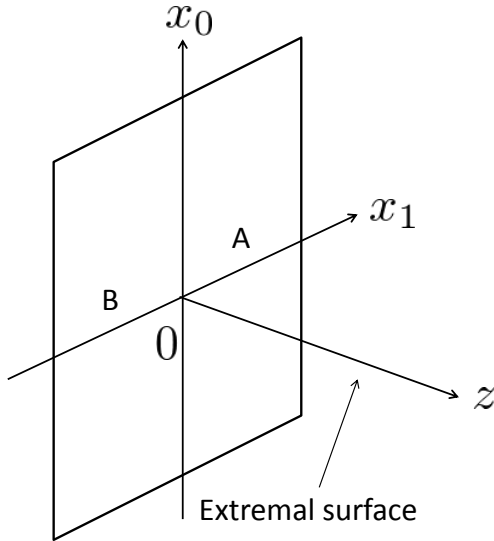
Figure 3.7: Set-ups of a half plane and extremal surface in AdS spacetime. We omit other directions.
