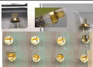
Fig.1 Diamond detectors.
