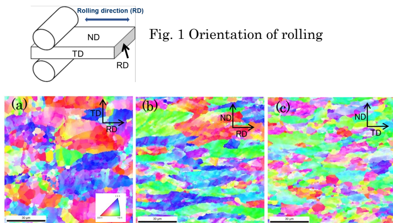
Fig. 2. IPF-map(ND) (a):ND, (b):TD, (c):RD
