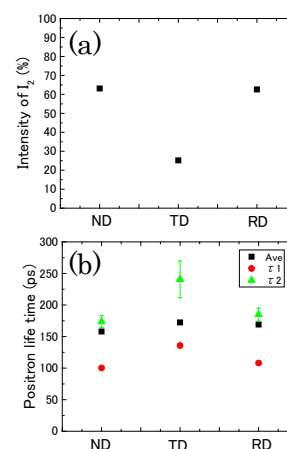
Fig. 3. Intensity of I_2 (a) and positron life time(b).
