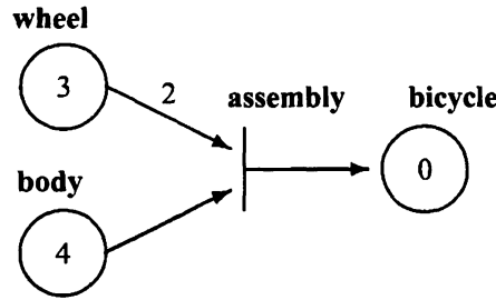
Figure 1. Graphical representation of a Petri net
