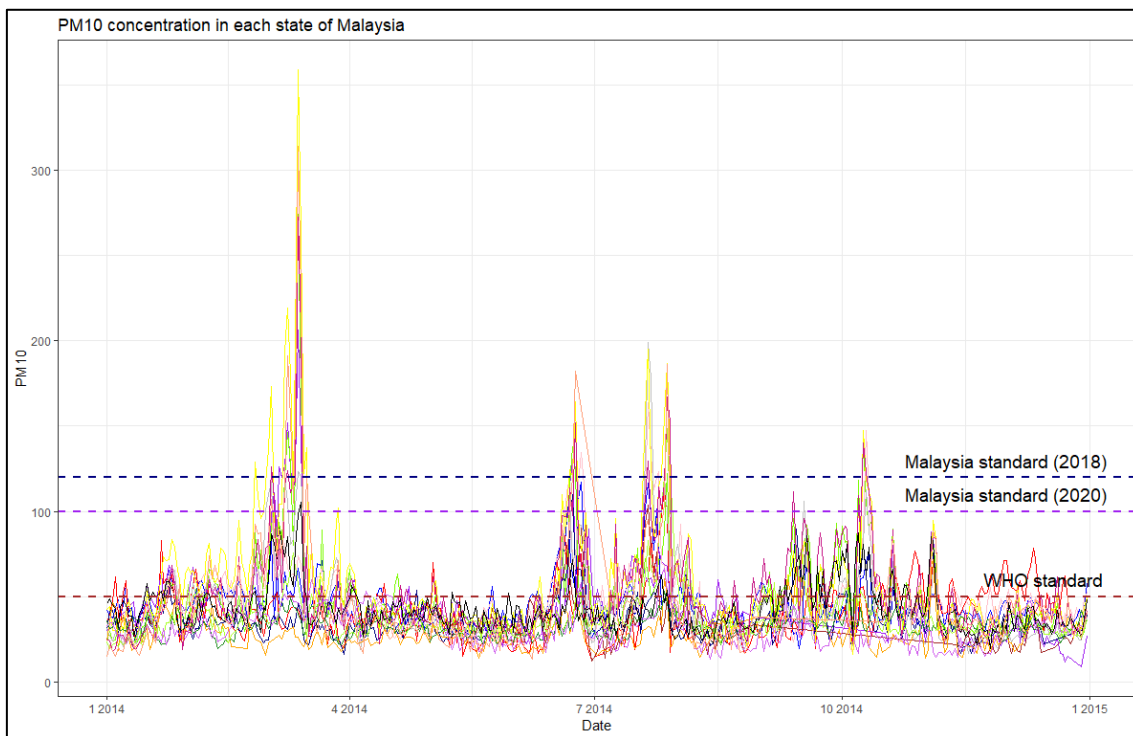
Figure 4.2. Concentration of \text{PM}_{10} over time for all states in Malaysia in 2014.
