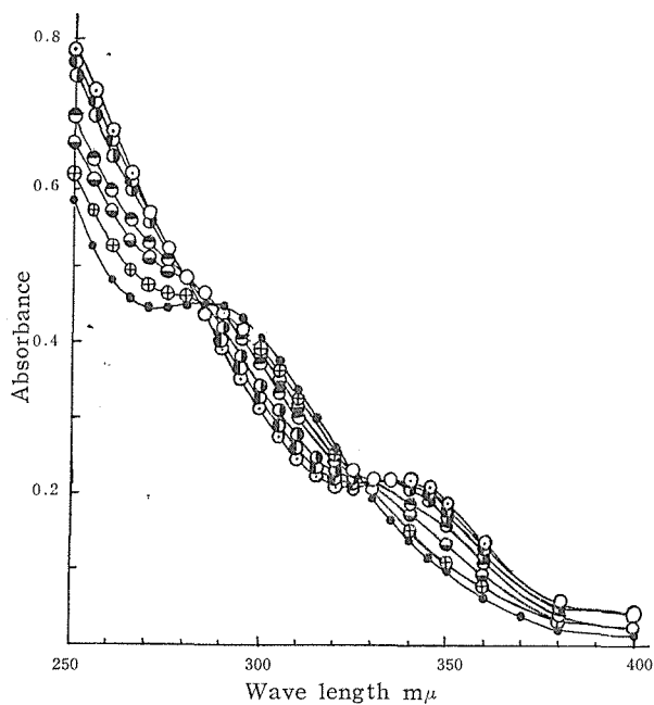
Fig. 5-b. Absorption spectra of ferric acetate in 10 M acetic acid (2). Fe, 10 p.p.m. —●— \text{HClO}_4 , 0.1 N. pH : —⊕— 0.40, —●— 0.50, —●— 0.60, —●— 0.80, —●— 1.00, —⊙— 1.21.
