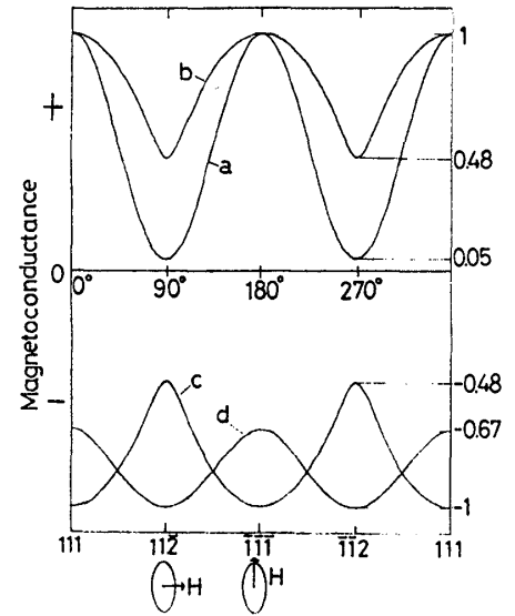
Fig.8 Theoretical predictions of magnetoconductance anisotropy of 1-valley Ge. The magnetic field is rotated in the plane (110). The meaning of each curves is as follow; (a):localization theory in low H, (b): localization theory in high H, (c):orbital term of interaction theory in high H and (d):spin-Zeeman term of interaction theory in high H. Magnetoconductance is isotropic in the plane (111).
