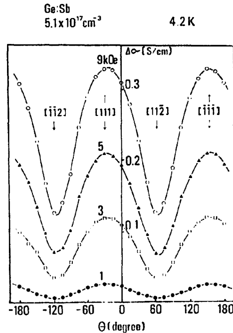
Fig.7 Anisotropy of positive magnetoconductance of 1-valley Ge with N=5.1 \times 10^{17} \text{ cm}^{-3} at 4.2K. The conductivity is measured along [111] and the magnetic field is rotated in the plane of (1\bar{1}0) .
