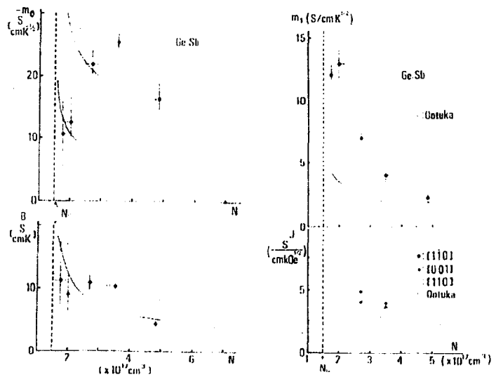
Fig.2 Donor concentration dependence of fitted values of m_0 , m_1 , J and B in Eqs.(2) and (3). The solid curves are the theoretical predictions.
