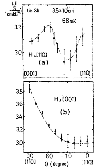
Fig.5 Anisotropy of negative magnetoconductance of the sample with N = 3.5 \times 10^{17} \text{ cm}^{-3} at 68mK. The current is along [1\bar{1}0] and H is rotated in the plane (1\bar{1}0) in (a), and (001) in (b).
