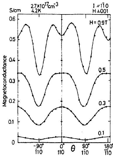
Fig.3 Anisotropy of positive magnetoconductance of the sample with N = 2.7 \times 10^{17} \text{ cm}^{-3} . The conductivity is measured along [1\bar{1}0] and the magnetic field is rotated in the plane (001).
