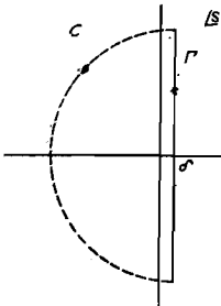
Fig. 1. Integration path in complex plane s .
