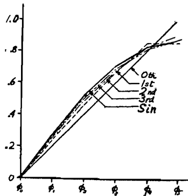
Fig. 24. Approximation for eigenfunction of case (A).
