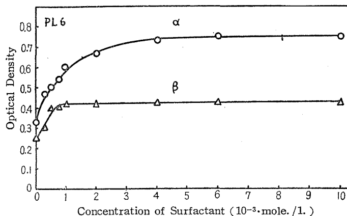
Fig. 5. Relation between concentration of non-ionic surfactant (PL6) and optical density of two characteristic bands.
