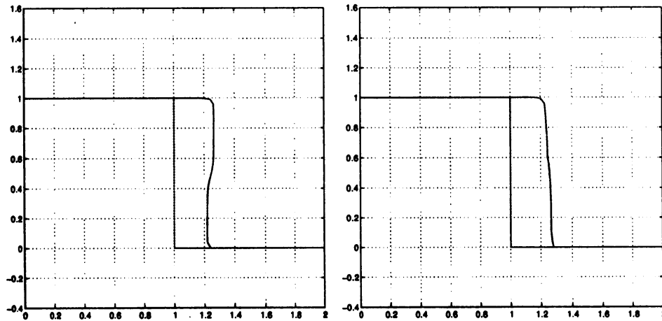
Figure 7: Numerical solution to the Riemann problem of Burgers' Equation with u_L = 1.0 , u_R = 0.0 . We plotted the zero level sets at time t = 0 and 0.5 obtained from M = 0.04 and 1.0.
