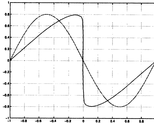
Figure 9: Numerical solution (WENO5-LLF) to the Burgers Equation with sine wave as initial data. We plotted the zero level set at time t = 0 and 0.5.
