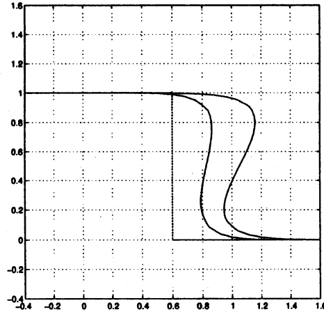
Figure 3: Numerical solution to the Riemann problem for equation (4) with u_L = 1.0 , u_R = 0.0 , and a = 0.1 . We plotted the zero level set at time t = 0, 0.5 , and 1.0 .
