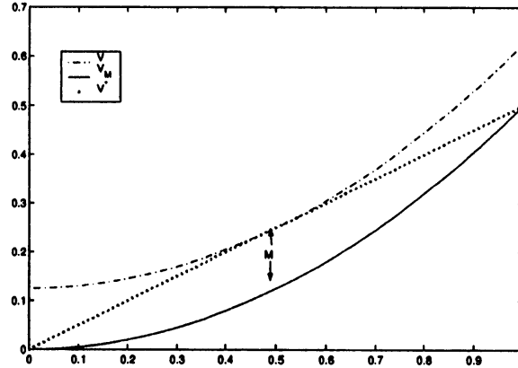
Figure 4: V(y) = y^2/2 on [0, 1] . The minimum value of M should be 1/8 .
