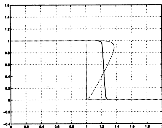
Figure 8: Numerical solution to the Riemann problem of Burgers' Equation with u_L = 1.0 , u_R = 0.0 . We plotted the zero level sets at time t = 0 and 0.5 obtained from M = 0.2 and 0.0.
