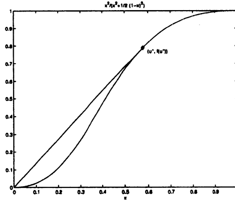
Figure 1: The concavification of the flux in Buckley-Leverett equation
