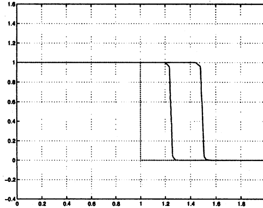
Figure 6: Numerical solution (WENO5-LLF) to the Riemann problem of Burgers' Equation with u_L = 1.0 , u_R = 0.0 , and M = 0.2 . We plotted the zero level set at time t = 0, 0.5 , and 1.0 .
