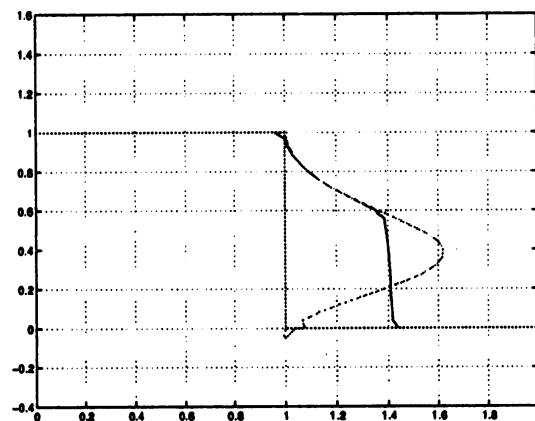
Figure 11: Numerical solution to the Riemann problem of the Buckley-Leverett Equation with u_L = 1.0 , u_R = 0.0 and a = 0.5 . We plotted the zero level sets at time t = 0 and 0.3 obtained from M = 0.2 and 0.0 . The little fragment of contour at the lower part of the jump is due to the contour plotter.
