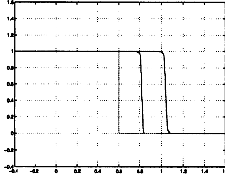
Figure 5: Numerical solution to the Riemann problem for equation (4) with u_L = 1.0 , u_R = 0.0 , a = 0.1 , and M = 0.2 . We plotted the zero level set at time t = 0, 0.5 , and 1.0 .
