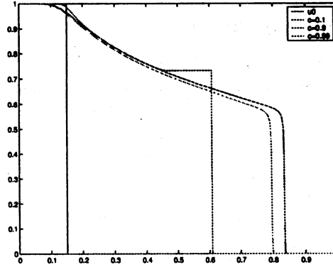
Figure 12: The numerical solutions of the Buckley-Leverett equation in non-conservative form obtained from the monotone Lax-Friedrichs scheme (13). The approximations are computed to t = 0.1 on [0, 1] with 2,500 grid points.
