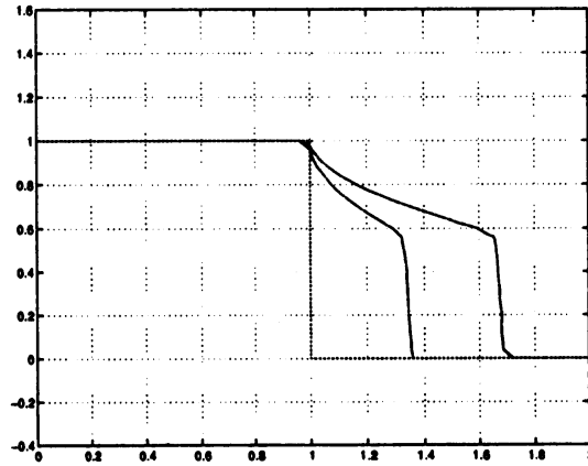
Figure 10: Numerical solution to the Riemann problem of the Buckley-Leverett Equation with u_L = 1.0 , u_R = 0.0 and a = 0.5 . We plotted the zero level set at time t = 0, 0.25 , and 0.5 .
