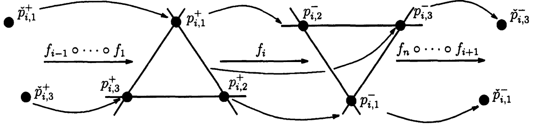
図 5: The points p_{i,\ell}^+ \in I(f) and p_{i,\ell}^- \in I(f^{-1})
