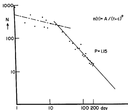
Fig. 4 Decrease rate of after-shocks.
