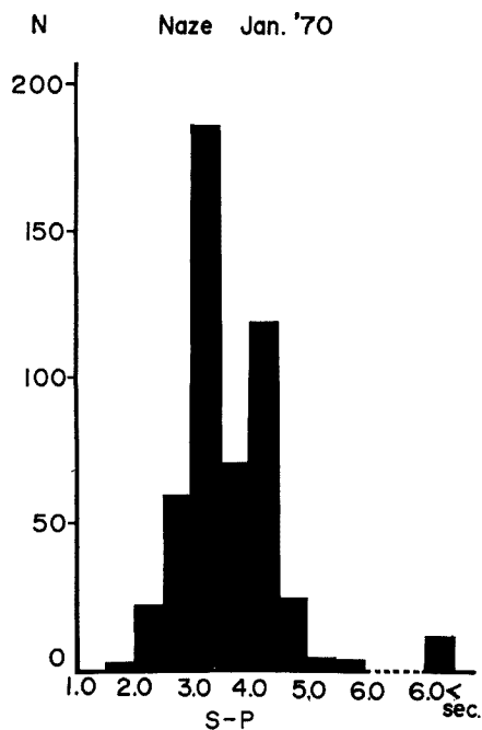
Fig. 5 Frequency distribution of S-P time in Jan., 1970.
