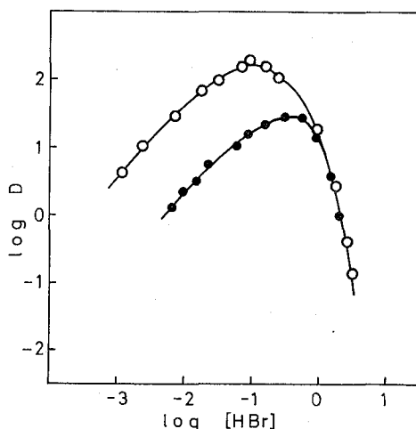
Fig. 3. The distribution ratio of zinc (—○—) and cadmium (—●—) as a function of hydrogen bromide concentration.
