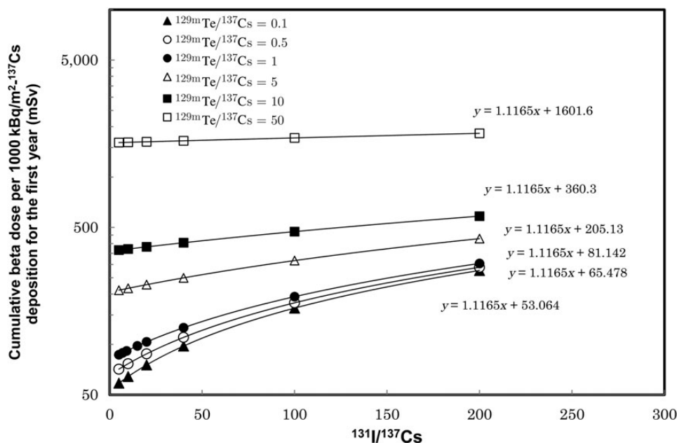
Fig. 3. Cumulative \beta -ray dose per ^{137}\text{Cs} deposition of 1000 \text{ kBq/m}^2 for the first year as a function of ^{131}\text{I}/^{137}\text{Cs} and ^{129\text{m}}\text{Te}/^{137}\text{Cs} ratio.
