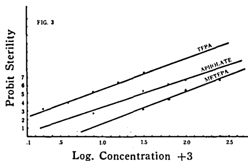
Fig. 3. Susceptibility of M. d. nebulosa to apholate, tepa and metepa when acetone solutions of these chemicals were applied topically to the dorsum of individual flies.
