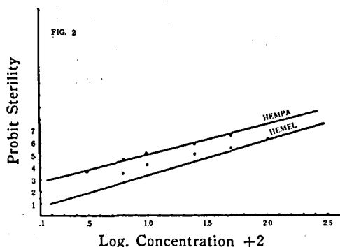
Fig. 2. Susceptibility of M. d. nebulosa to hempa and hemel administered in the food of adults.
