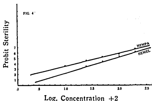
Fig. 4. Susceptibility of M. d. nebulosa to hempa and hemel when acetone solutions of these chemicals were applied topically to the dorsum of individual flies.
