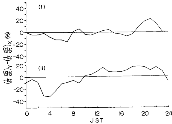
Fig. 7. Differences of variations of columnar resistances at the two stations for the periods of I and II obtained from the calculation: \left(\frac{1}{i} \frac{di}{dt}\right)_X - \left(\frac{1}{i} \frac{di}{dt}\right)_Y = \left(\frac{1}{R} \frac{dR}{dt}\right)_Y - \left(\frac{1}{R} \frac{dR}{dt}\right)_X
