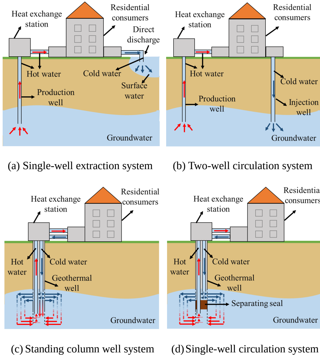
Fig. 3 Schematic diagrams of hydrothermal type geothermal systems
