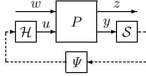
FIG. 1. Sampled-data system \Sigma_{\text{SD}} .
