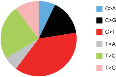
Mutation spectrum in CCHD-PPGL
