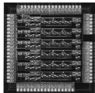
Figure 2. The layout of the waveform receiver.
