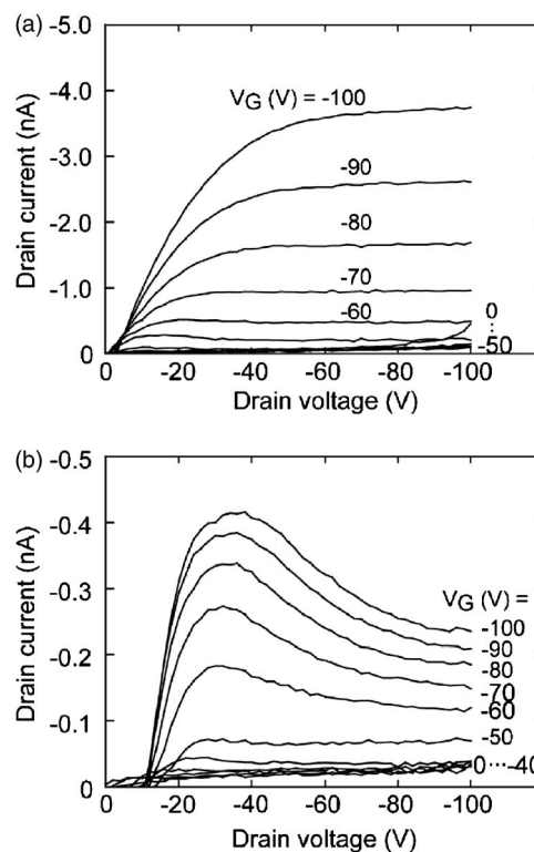
FIG. 4. FET characteristics of \text{Alq}_3 -based ambipolar OFET with HMDS-treated \text{SiO}_2/p^+ \text{Si} substrate with bottom-contact electrodes of Au/Cr (channel width of 76 \text{ mm} and channel length of 25 \text{ }\mu\text{m} ) obtained in (a) vacuum of 1 \times 10^{-5} Pa and (b) air.
