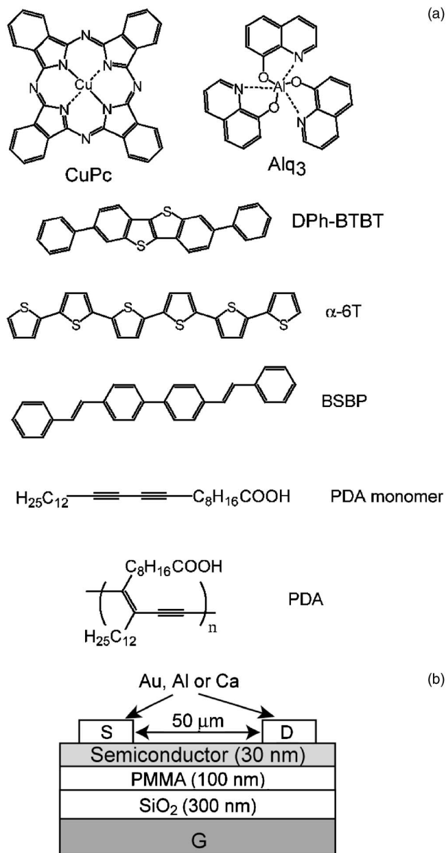
FIG. 1. (a) Molecular structures of organic semiconductors used. (b) Schematic view of OFET device structure.
