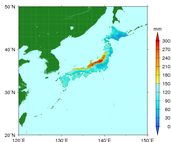
Fig. 6b Monthly mean precipitation for January from the AGCM20 output for 1979~2003
