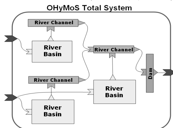
Fig. 8 Example of OHyMoS composed by several elements for rainfall-runoff simulation, channel routing simulation, and dam reservoir-operating simulation.
