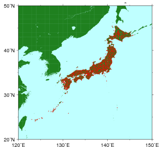
Fig. 3 AMeDAS observation points throughout Japan composing more than 1,300 stations
