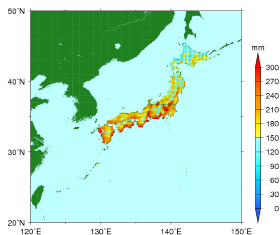
Fig. 6d Monthly mean precipitation for August from the AGCM20 output for 1979~2003
