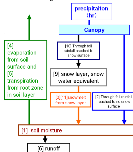
Fig.2 Structure of hydrologic output data from AGCM20
