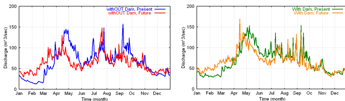
Fig. 16 Simulated annual discharge pattern of present and future without dam reservoir operations (left) and with the dam reservoir operations (right). It is able to see the changed flow pattern of future was regulated through the designed dam reservoir operation, and the future flow pattern got close to the present flow pattern (Yukatahara Outlet: 1677.5 km 2 ).
