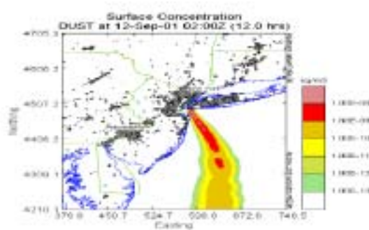
Fig. 7: Plume Analysis
