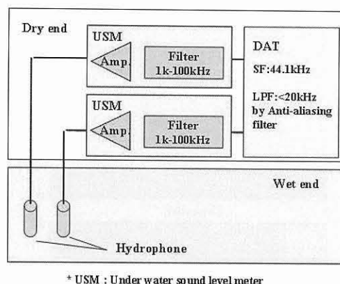
Fig. 2. Block diagram of the recording system.
