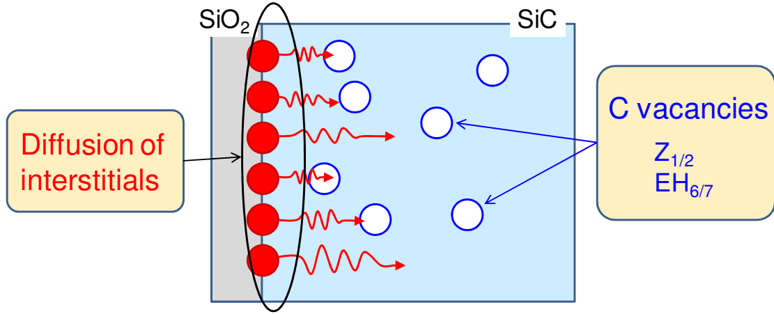
Figure 5.1: Schematic model for the reduction of the Z_{1/2} and EH_{6/7} centers during oxidation. Interstitials generated at the SiO 2 /SiC interface diffuse into SiC bulk and occupy carbon vacancies related to the Z_{1/2} and EH_{6/7} centers.
