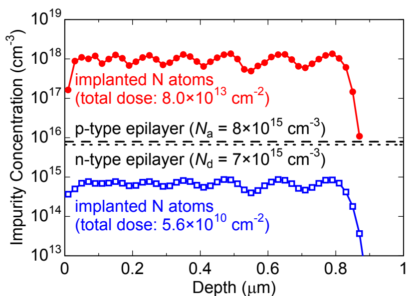
Figure 3.2: Depth profiles of implanted N atoms simulated by TRIM code (filled circles: high-dose-implanted N atoms, squares: low-dose-implanted N atoms, dotted/dashed lines: doping levels in n -/ p -type starting materials).
