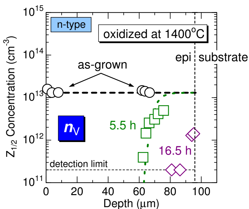
Figure 5.14: Depth profiles of the Z_{1/2} center after oxidation at 1400^\circ\text{C} for 5.5 h and 16.5 h. The dotted line indicates the n_V profile after 5.5-h oxidation calculated with the parameters in Table 5.2 and each symbol indicates the experimental data. The calculated line for 16.5-h oxidation is not shown because the n_V is lower than 1 \times 10^{10} \text{ cm}^{-3} in the 96- \mu\text{m} -thick epilayer.
