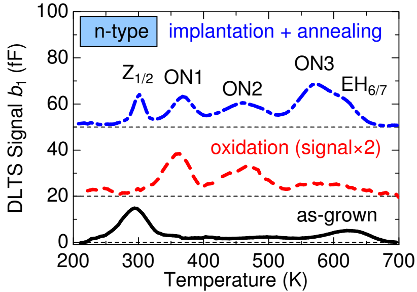
Figure 5.2: DLTS spectra of the n -type 4H-SiC after thermal oxidation at 1300°C for 1.3 h (dashed line) and C + implantation followed by Ar annealing at 1800°C for 20 min (dashed-dotted line).
