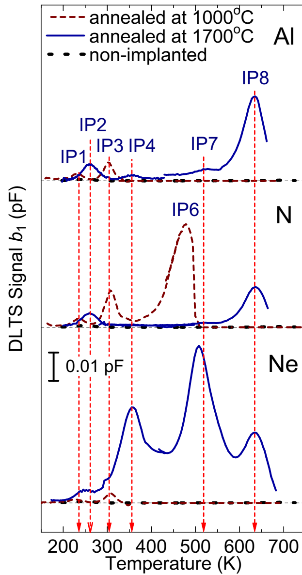
Figure 3.8: DLTS spectra of p -type 4H-SiC implanted with \text{Al}^+ , \text{N}^+ , and \text{Ne}^+ (implant dose: 5.6 \times 10^{10} \text{ cm}^{-2} ) annealed at 1000°C (dashed line) and 1700°C (solid line). The spectrum of nonimplanted sample is indicated with a dotted line.
