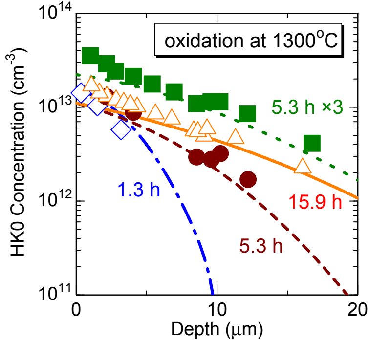
Figure 7.12: Depth profiles of the HK0 center after oxidation at 1300°C for 1.3–15.9 h. Each symbol indicates experimental data and each line indicates the calculated n_I distribution obtained from Eqs. (5.1)–(5.7).
