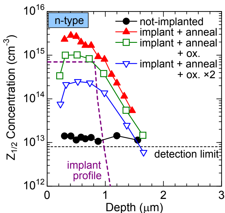
Figure 4.2: Depth profiles of the Z_{1/2} center observed in nonimplanted (filled circles) and \text{Al}^+ -implanted n -type 4H-SiC after Ar annealing at 1700°C for 30 min (filled triangles) and after the annealing followed by oxidation at 1150°C (squares and inverse triangles).
