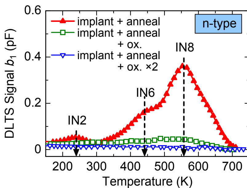
Figure 4.3: DLTS spectra of high-dose \text{P}^+ -implanted n -type 4H-SiC after Ar annealing at 1700°C for 30 min (filled triangles) and after the annealing followed by oxidation at 1150°C (squares and inverse triangles).
