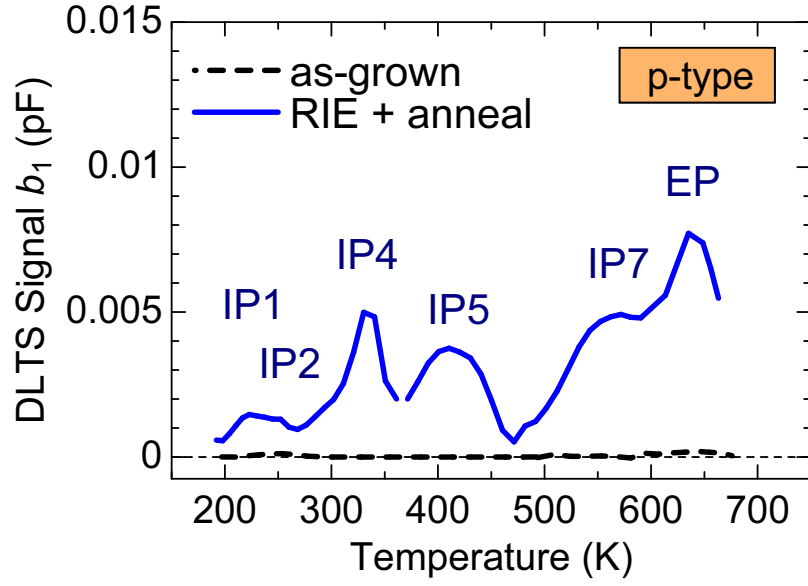
Figure 3.17: DLTS spectra obtained from as-grown (dashed line) and RIE-etched p -type 4H-SiC with annealing at 1000°C (solid line).
