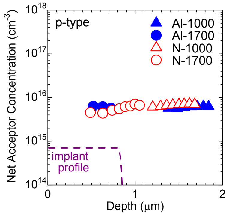
Figure 3.7: Depth profiles of net acceptor concentration (Al-1000: \text{Al}^+ -implanted sample annealed at 1000^\circ\text{C} , Al-1700: \text{Al}^+ -implanted sample annealed at 1700^\circ\text{C} , N-1000: \text{N}^+ -implanted sample annealed at 1000^\circ\text{C} , N-1700: \text{N}^+ -implanted sample annealed at 1700^\circ\text{C} ). The high-resistance region does not exist in the sample annealed at 1700^\circ\text{C} .
