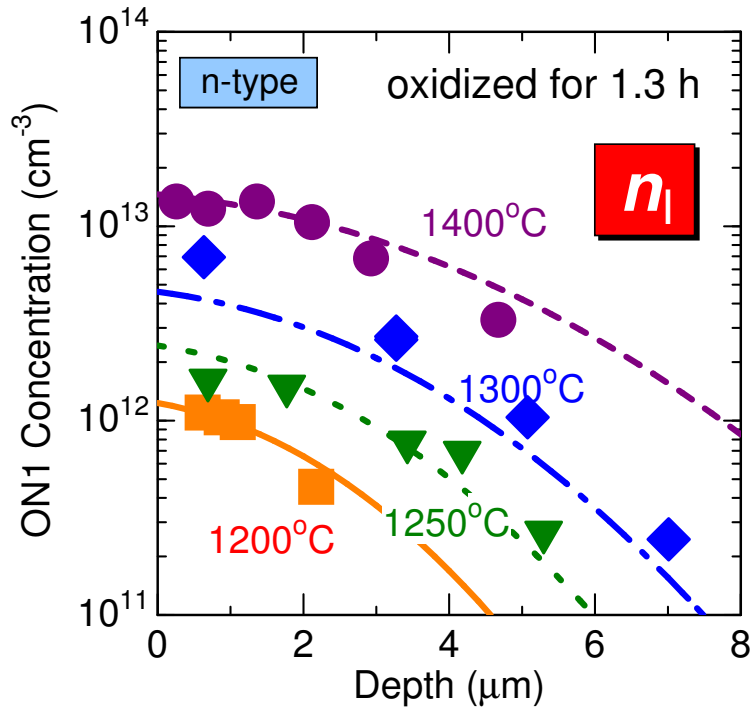
Figure 5.4: Depth profiles of the ON1 center after oxidation at various temperatures for 1.3 h. Each symbol indicates the experimental data and each line indicates the calculated n_I distribution obtained from Eqs. (5.1)–(5.8).
