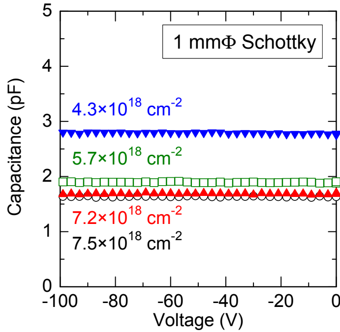
Figure 6.2: C - V characteristics at room temperature (RT) of the D samples irradiated by low-energy (250 keV) electrons with various fluences (circles: 7.5 \times 10^{18} \text{ cm}^{-2} , triangles: 7.2 \times 10^{18} \text{ cm}^{-2} , squares: 5.7 \times 10^{18} \text{ cm}^{-2} , reverse triangles: 4.3 \times 10^{18} \text{ cm}^{-2} ).
