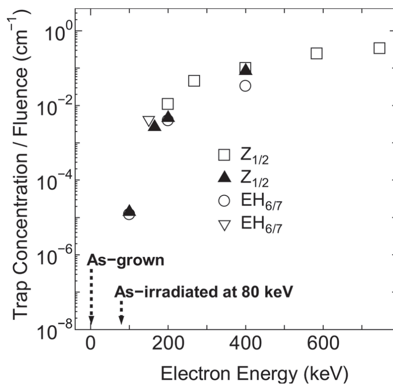
Figure 8.2: Z_{1/2} and EH_{6/7} concentrations in electron-irradiated 4H-SiC normalized by the electron fluence vs the electron energy [12].
