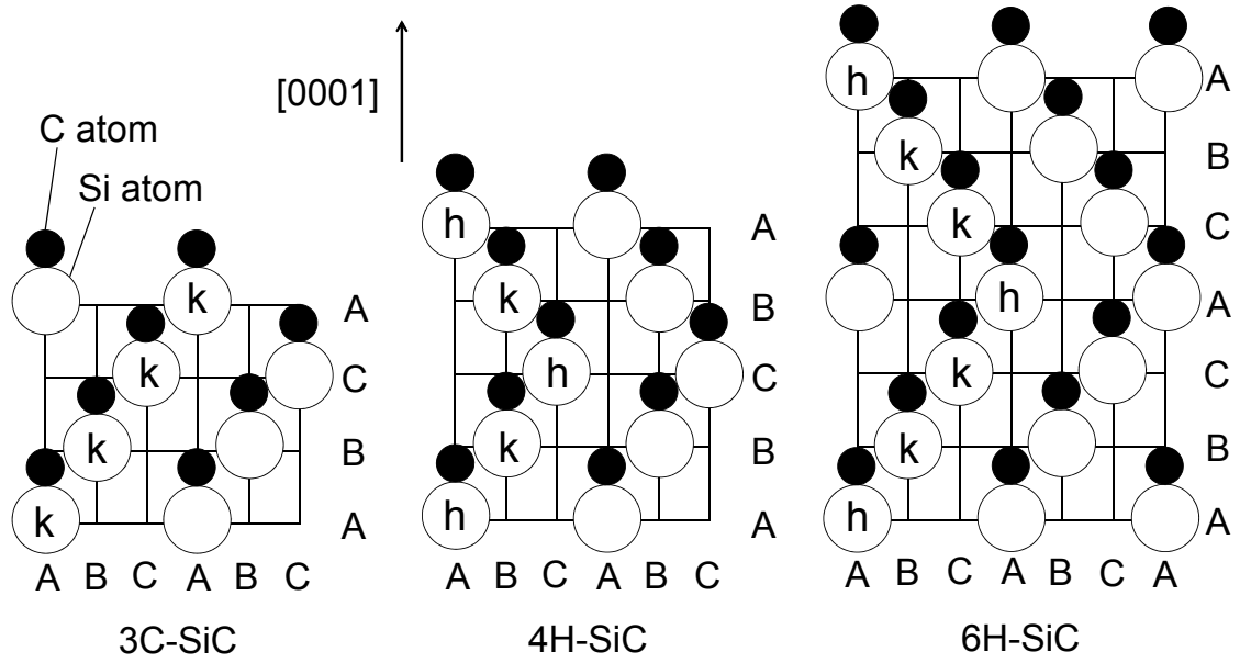
Figure 1.3: Schematic crystal structures of major SiC polytypes. SiC has three possible occupation sites denoted by A, B, and C, which are also categorized as cubic site (k) or hexagonal site (h).
