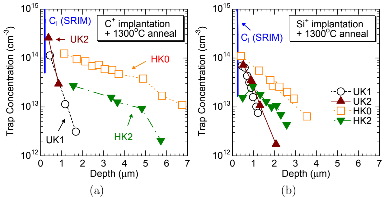
Figure 7.22: Depth profiles of deep levels in the p -type 4H-SiC after (a) C^+ and (b) Si^+ implantation (dose: 1.4 \times 10^{13}\ \text{cm}^{-2} ) followed by Ar annealing at 1300^\circ\text{C} for 20 min. A depth profile of carbon interstitials just after C^+ implantation simulated by SRIM code is also shown as a solid line.
