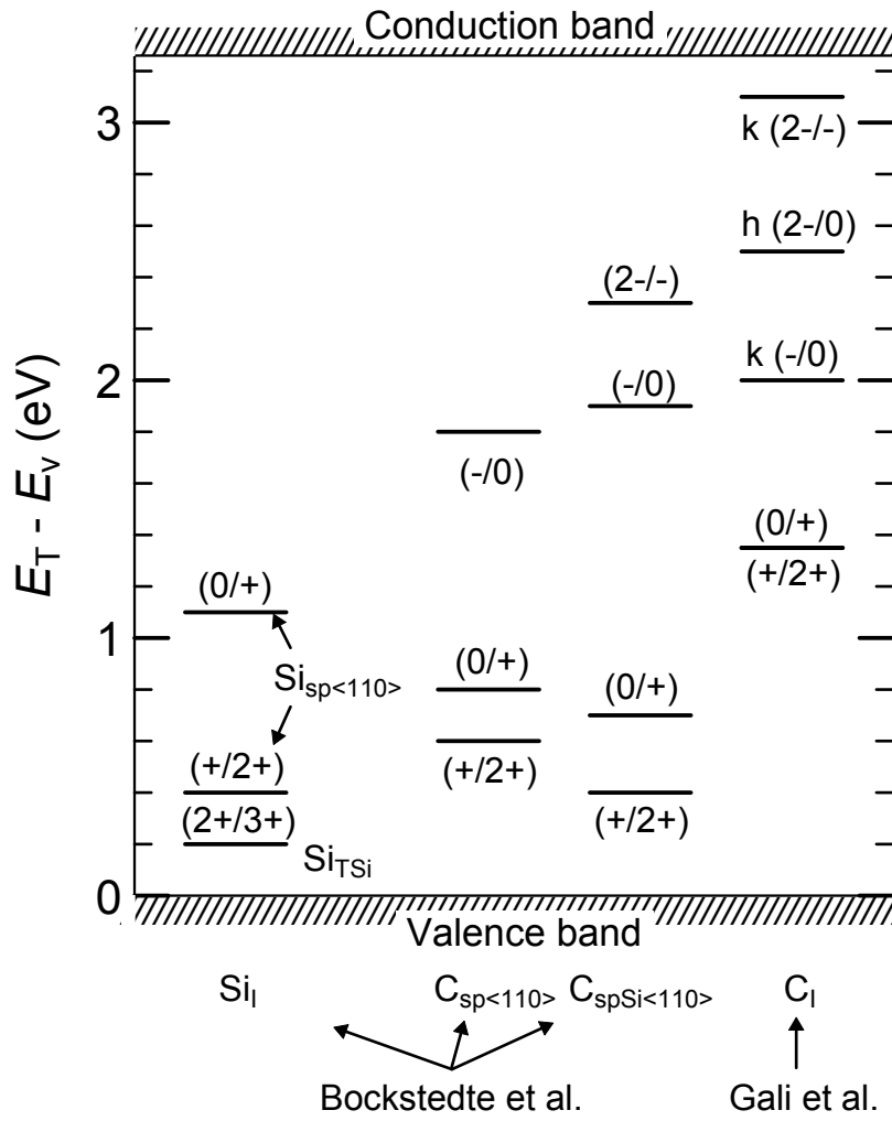
Figure 7.14: Energy levels of silicon interstitial ( \text{Si}_\text{I} ) and carbon interstitial ( \text{C}_\text{I} ) obtained by ab initio calculation [19, 20].
