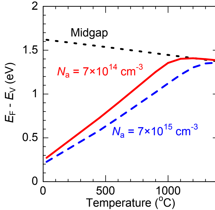
Figure 7.13: Temperature dependence of the Fermi level in p -type 4H-SiC with different acceptor concentration.
