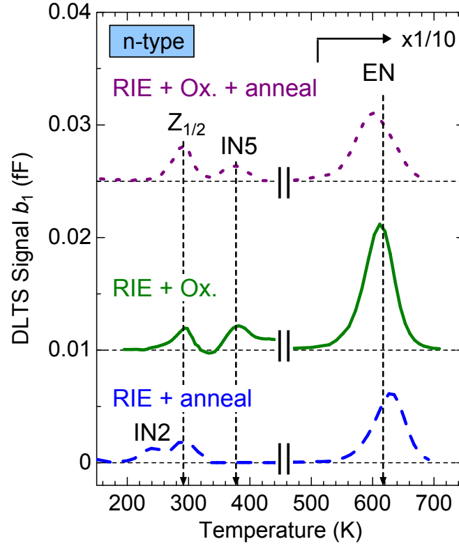
Figure 4.8: DLTS spectra obtained from RIE-etched n -type 4H-SiC after Ar annealing at 1000°C for 30 min (dashed line), after oxidation at 1100°C for 30 min (solid line), and after the oxidation followed by Ar annealing at 1400°C for 30 min (dotted line).
