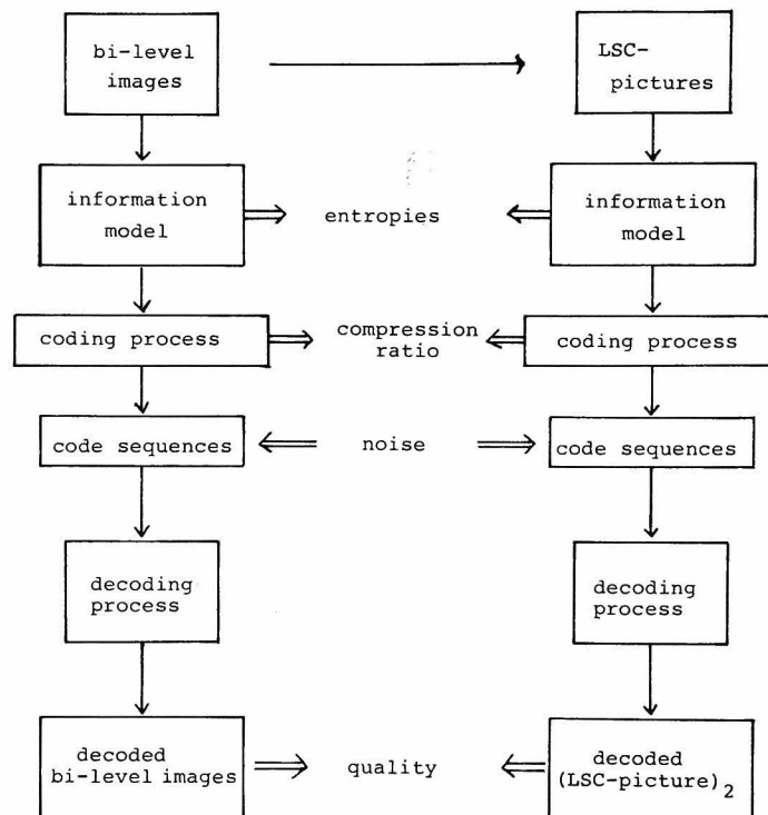
Fig.4-67 Simulation system.
