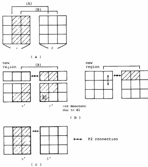
Fig.4-22 Explanation of the proof for Theorem 4-4 (necessity).
