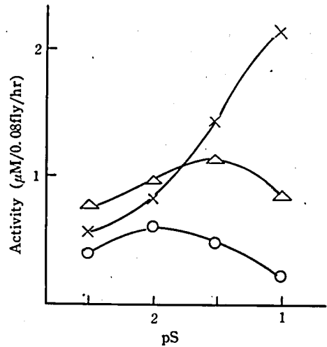
Fig. 4 Hydrolysis of acetylcholine (O), propionylcholine ( \Delta ) and butyrylcholine (X) by cholinesterase of the housefly.
