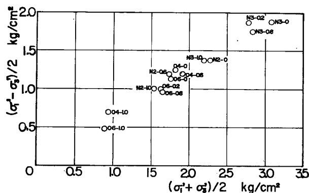
Fig. 8 Relationship between strength and normal stress at failure.
