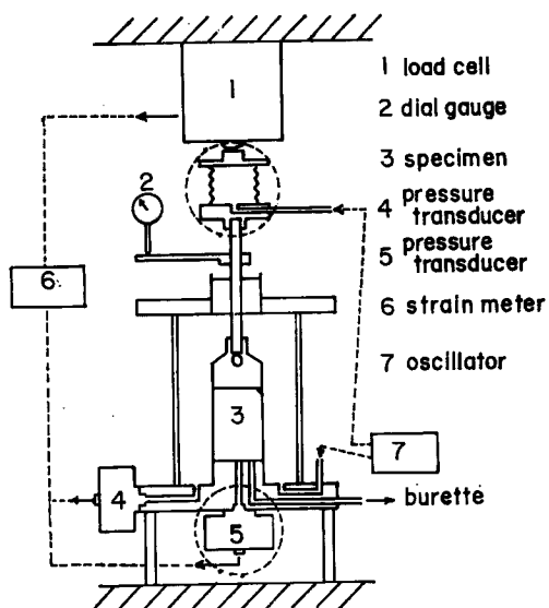
Fig. 1 Triaxial cell.
