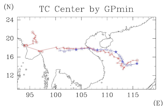
Fig. 3. Typhoon Lekima center position tracks. Blue line is the best track data by RSMC Tokyo, and red line is the minimum pressure center in the model.
