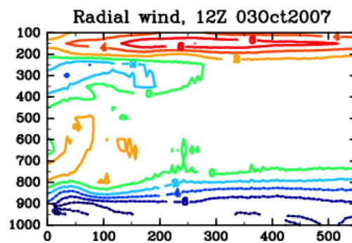
Fig. 4. Vertical cross section of radial wind for Typhoon Lekima at 1200UTC 3 Oct. 2007. The origin of horizontal axis is the typhoon center. Cool color lines are inflow (negative) and warm color lines are outflow (positive).
