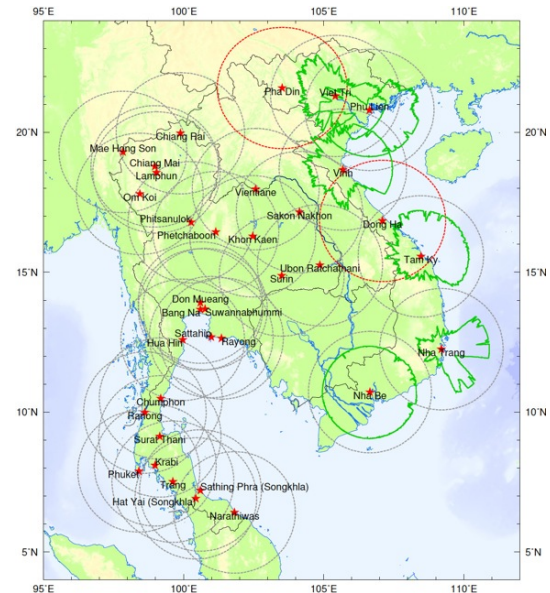
Fig. 1. Radar sites and their observation areas ( r < 250\text{km} ) in Indochina
