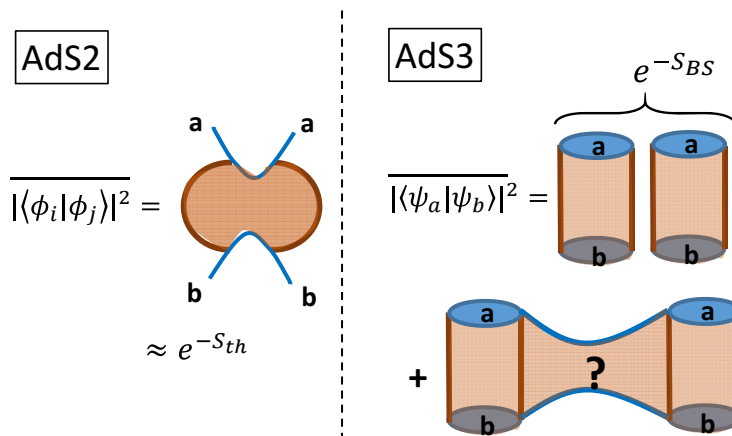
Figure 4. Gravity evaluations of the averages of squares of inner products in \text{AdS}_2 gravity (left) and \text{AdS}_3 gravity (right).
