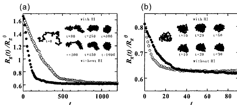
Figure 1: Temporal changes of the gyration radius R_g . (a) For a case where the initial R_g(0) is larger than R_g^0 . (b) For a case where the initial R_g(0) is smaller than R_g^0 . • and ○ correspond to the case with HI and without HI, respectively. Typical configurational changes of the polymer are also shown in the inset.
