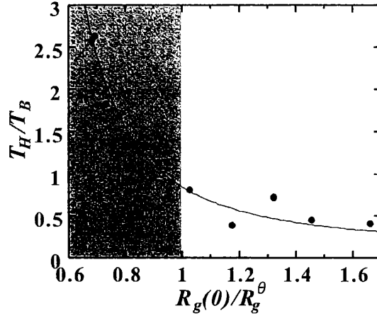
Figure 2: Variation of the ratio of T between T_H and T_B versus the scaled initial gyration radius R_g(0)/R_g^\theta
