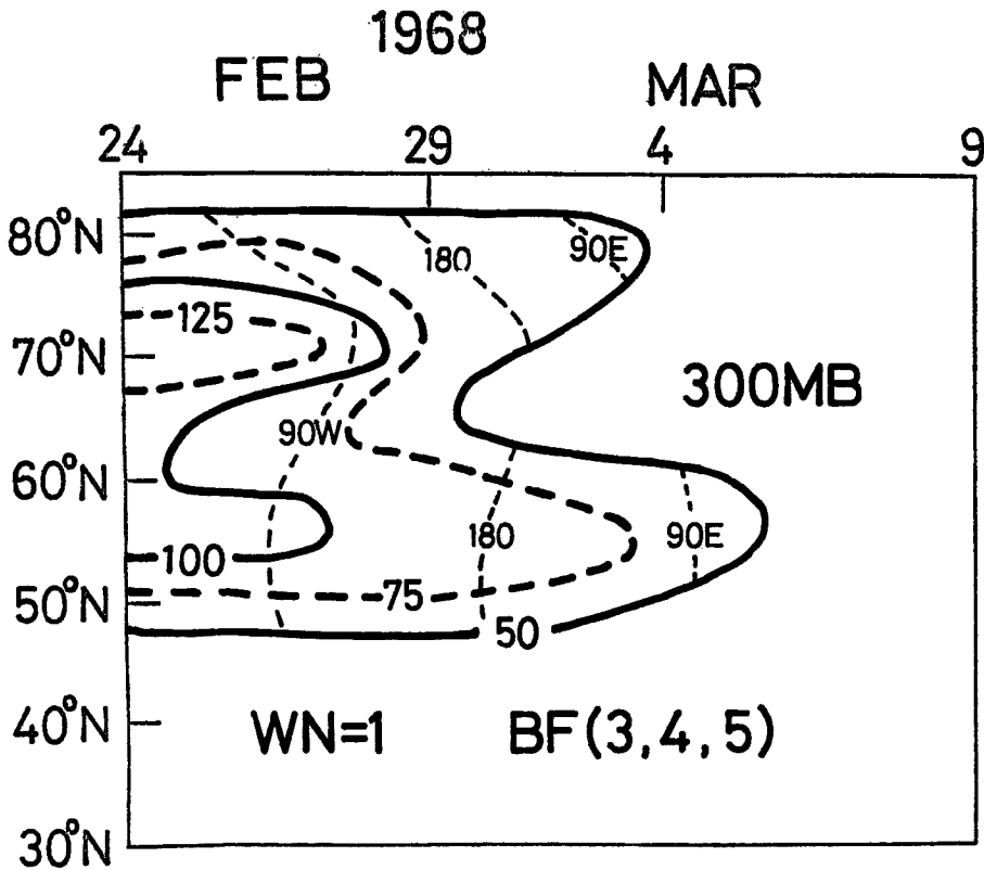
Fig. 7c The same as Fig. 7b, except for BF(3), (4) and (5).
